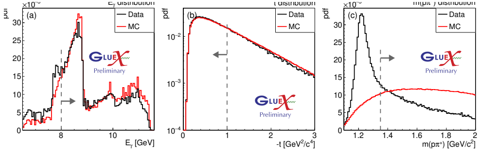
Figure 3. Basic distributions for MC versus real data with the applied event selection cuts indicated. Left: Distribution of the beam photon energy E_\gamma (a). Centre: Distribution of the momentum transfer -t . Right: Invariant mass of the (\pi p) system.
