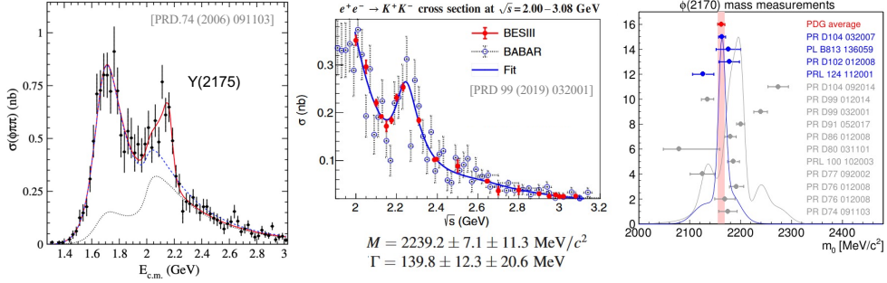
Figure 1. Left: Discovery plots by BaBar. Centre: A measurement by BESIII. Right: Compilation of individual measurements (not provided by PDG), summarised are all measurements listed by the PDG, and indicated by blue colour are those used by the PDG for their average values
