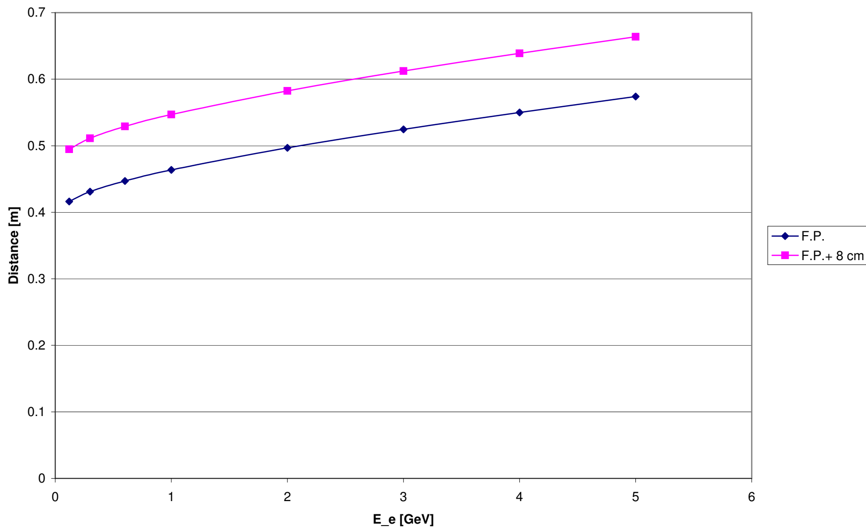
Distance from counter to magnet edge
