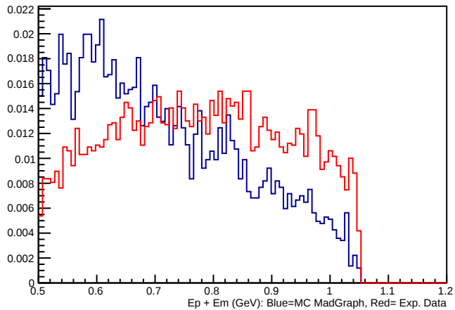
Ep+Em MadGraph
