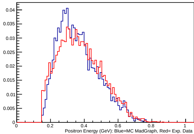
Ep+Em MadGraph
