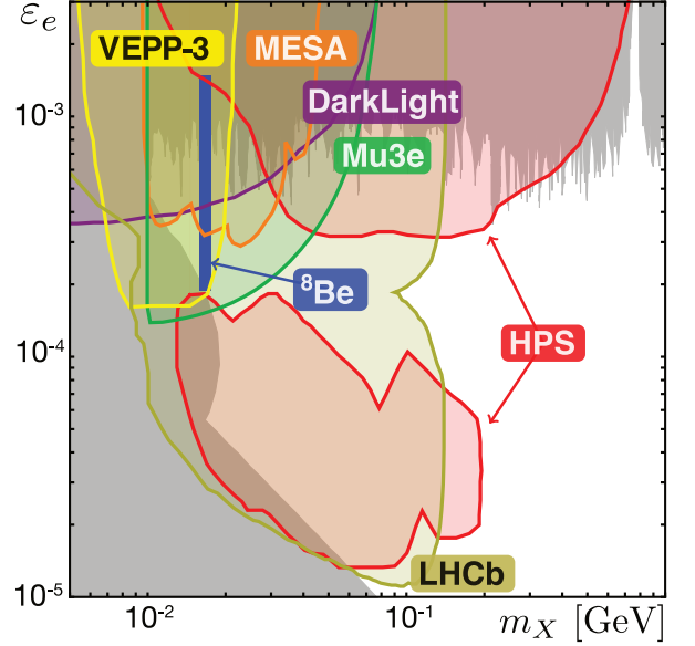
FIG. 2. The {}^8\text{Be} signal region, along with current constraints discussed in the text (gray) and projected sensitivities of future experiments in the (m_X, \varepsilon_e) plane. For the {}^8\text{Be} signal, the other couplings are assumed to be in the ranges given in Eq. (10); for all other contours, the other couplings are those of a dark photon.
