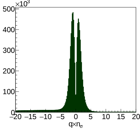
Figure 21: Distribution of q \times n_\sigma for in-time clusters, where q is the electric charge. Positive tracks were weighted by \approx 6 to have visually the same level as negatives.
