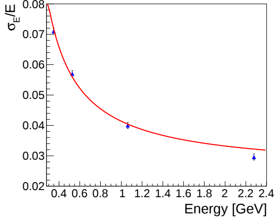
Figure 10: Energy resolution in the ECal as found in data by using elastically-scattered electrons and WAB events. The fit is given by Eq. 4 and only used data at 1.05 GeV beam energy. The point at 2.3 GeV was not included in the resolution fit; it was obtained using 2.3 GeV beam energy.
