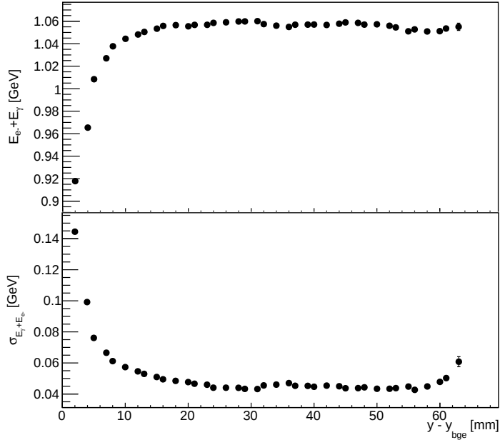
Figure 11: WAB events with |E_{e-} - E_{\gamma}| < 0.1 GeV. Top: energy sum (E_{e-} + E_{\gamma}) peak position. Bottom: energy sum peak standard deviation \sigma_{E_{e-} + E_{\gamma}}(y) as a function of vertical position of the electron across the ECal.
