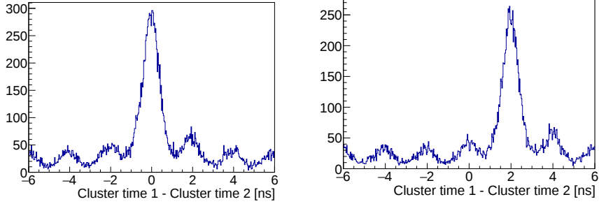
Figure 15: Time difference between the seed hits of two correlated clusters after finding initial RF offsets. Cluster 1 has a given (fixed over all events) seed crystal while cluster 2 may be anywhere in the ECal. The left and right plots show events for two different choices of seed crystals for cluster 1.
