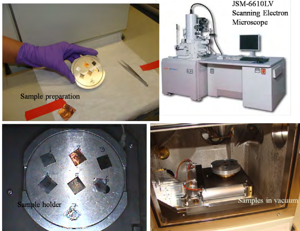
Figure E.2: Scanning Electron Microscopy (SEM) imaging setup.
