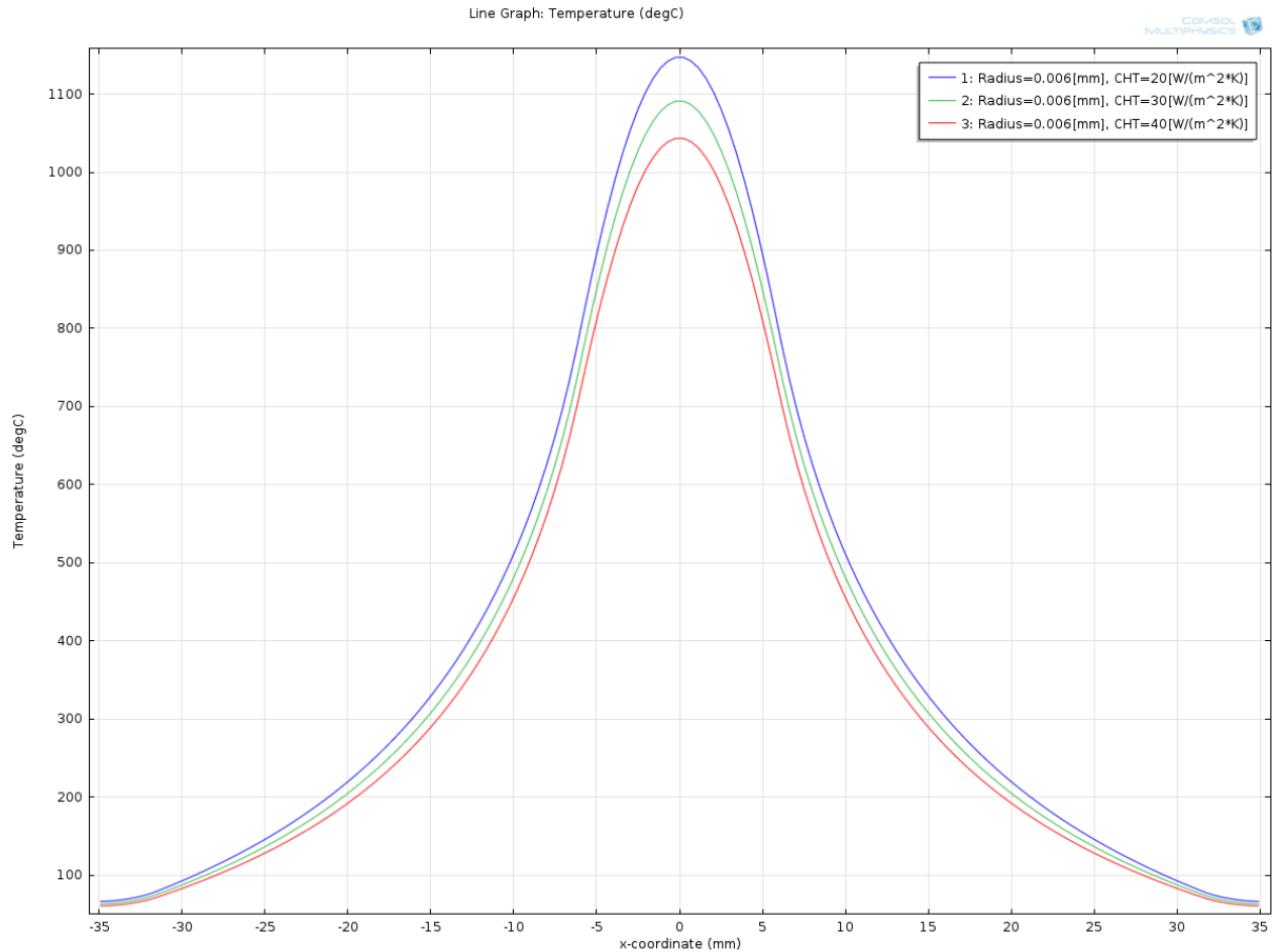
Figure 3. Beryllium exit window temperature in the CHT range 20-40 W/m 2 K at a beam radius of 6 mm
