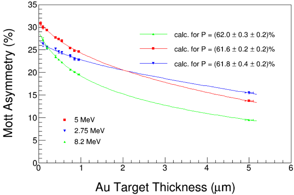
Figure 1. Asymmetry versus foil thickness measured at three different energies with the original version of the polarimeter. The fits to the data are based on a semi-empirical model developed by M. Steigerwald (S-1).
