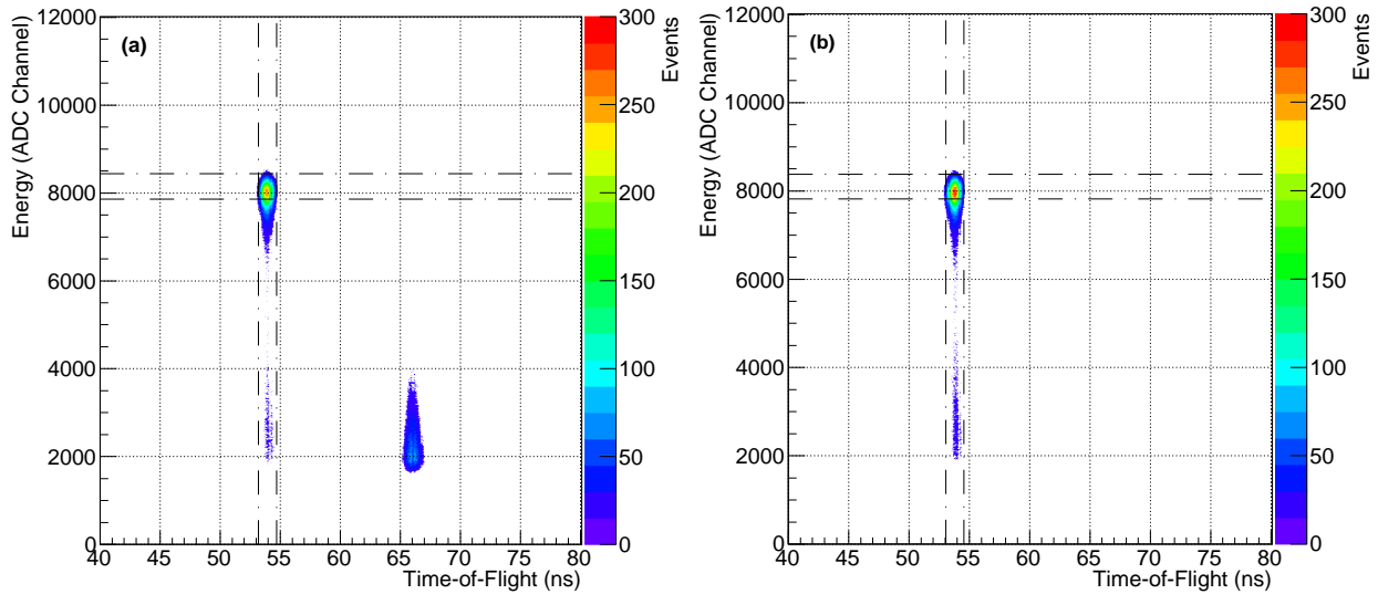
Figure 13. Energy-time coincidence plots show the distribution of events from a single Mott measurement in (a) Run 1 with the 350 nm foil where no hardware TOF veto was applied, and (b) Run 2 with the 350 nm where this hardware veto was applied. In each case the dashed lines indicate the applied TOF and Energy cuts that were used to select the events for the calculation of the asymmetry.
