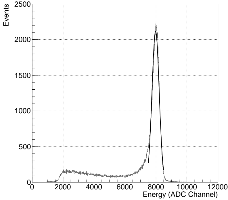
Figure 12. A Gaussian fit (solid line) to an energy spectrum of the E detector used to define the events used to calculate a Mott scattering asymmetry. Data from Run 1 with the 350 nm foil.
