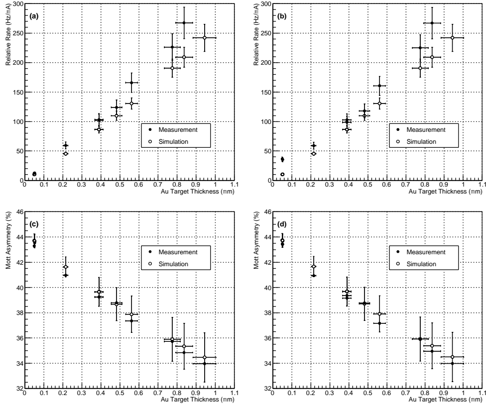
Figure 22. Measured counting rates compared to the GEANT4 simulation for a) Run 1 (U/D) b) Run 2 (L/R), and the measured asymmetry for c) Run 1 and d) Run 2, all versus FESEM measured foil thickness.
