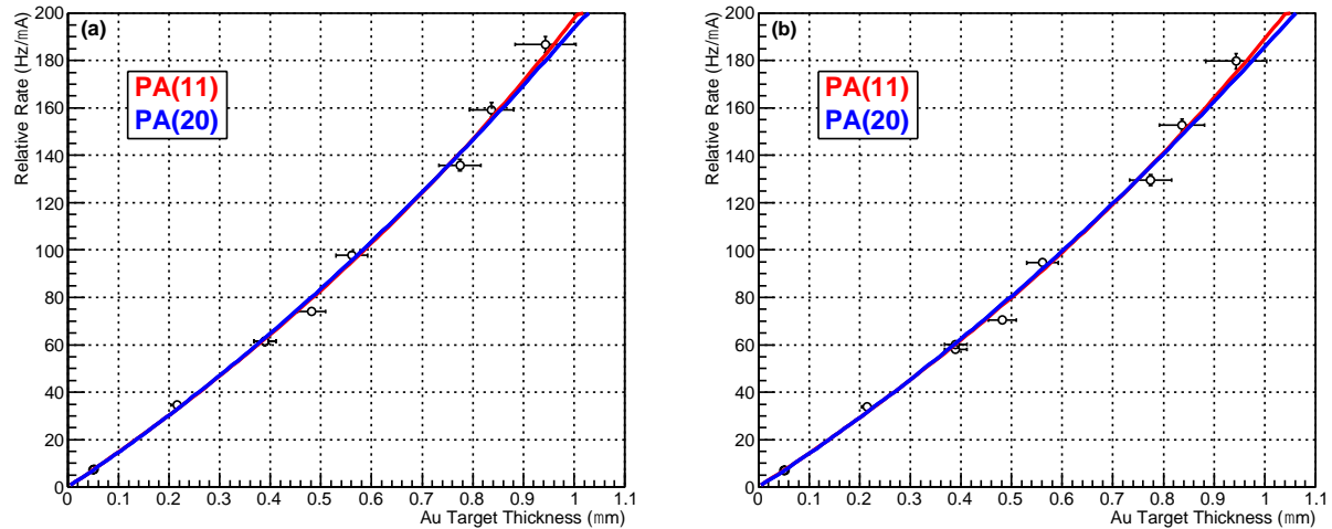
Figure 20. Normalized counting rate versus foil thickness for (a) Run 1 and (b) Run 2.
