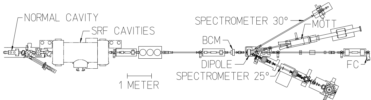
Figure 4. Plan view of the injector illustrating the RF accelerating cavities, the 12.5^\circ beam line through the Mott polarimeter, the spectrometer beam lines at -30^\circ and 25^\circ , and the straight beam line leading to the rest of the CEBAF injector including an RF cavity beam current monitor (BCM) and a Faraday cup (FC).
