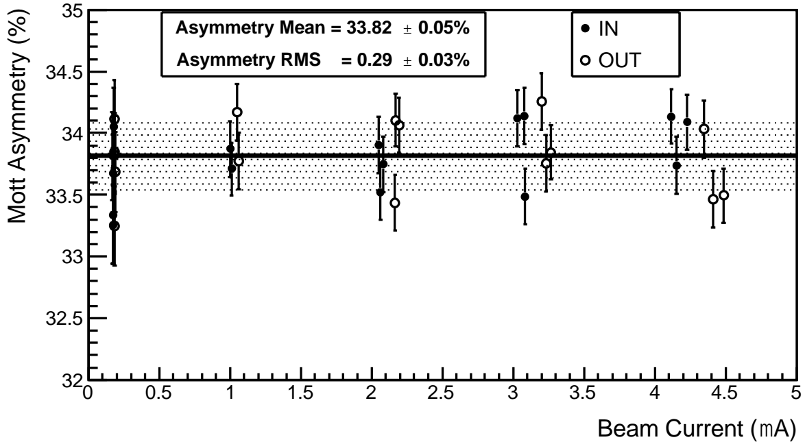
Figure 17. Mott asymmetry vs. beam current.
