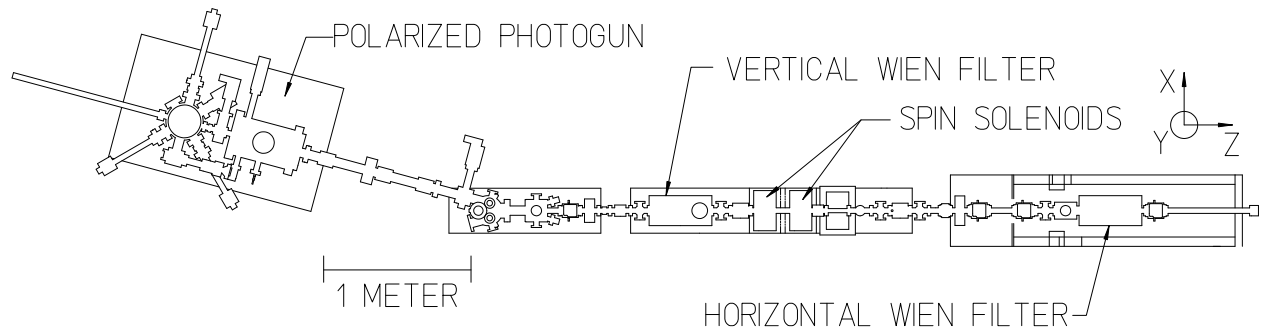
Figure 3. This plan view of the first part of the CEBAF injector highlights the polarized photogun followed by the electromagnetic elements that determine the spin direction of the beam. The orientation of the electron polarization is longitudinal as the beam exits the photogun.
