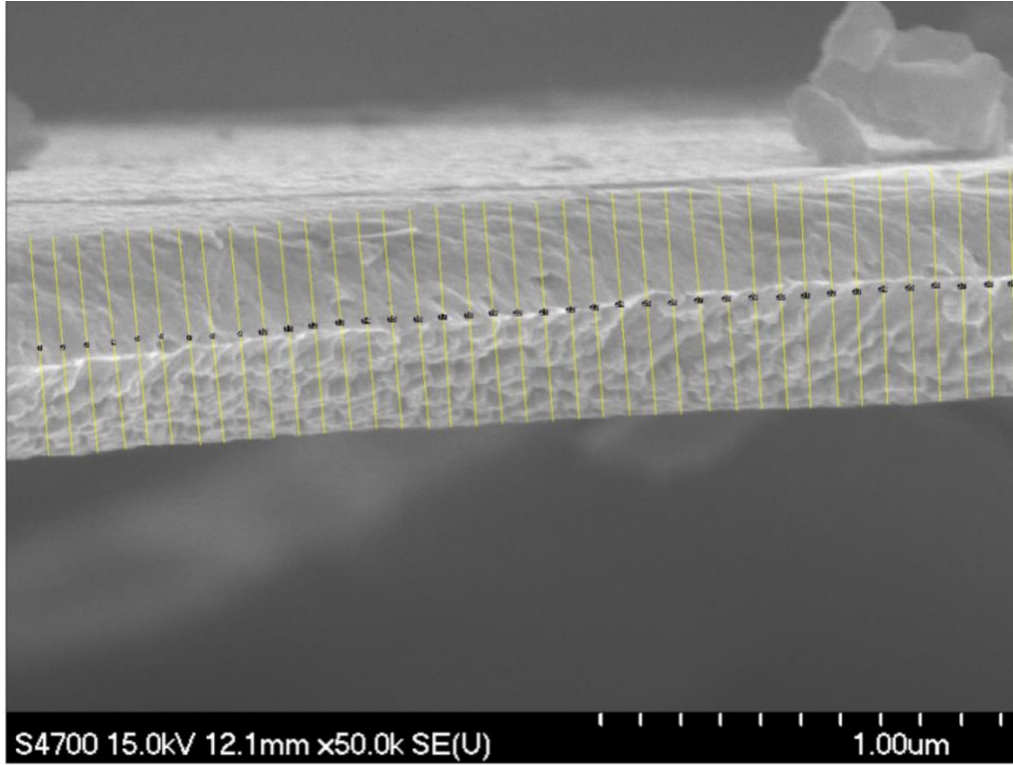
Figure A1. FESEM image of a nominal 625 nm thick gold foil mounted on a silicon substrate (lower dark region). Many measurements of the thickness along this region indicate the foil is 561.2 \pm 31.0 nm. Yellow lines with black labels denote the lines used for thickness analysis with ImageJ software (N-1).
