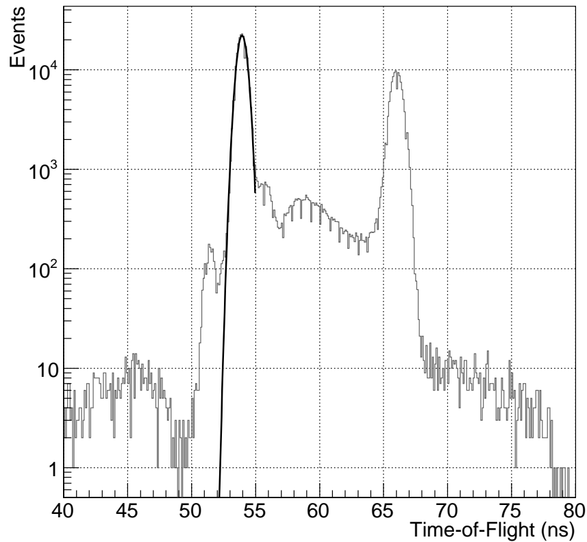
Figure 9. A typical time-of-flight distribution of Mott coincidence triggers. Mott events from the scattering foil appear at \sim 54 ns, while electrons backscattered from the beam dump are detected at \sim 66 ns. Data from Run 1 with the 350 nm foil.
