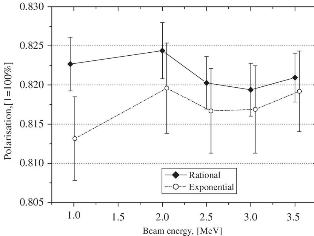
Figure 2. (excerpted from Ref. T-1) Polarized determination for several energies using two different fit functions. Errors ( \pm 2\sigma ) are fit uncertainties only.
