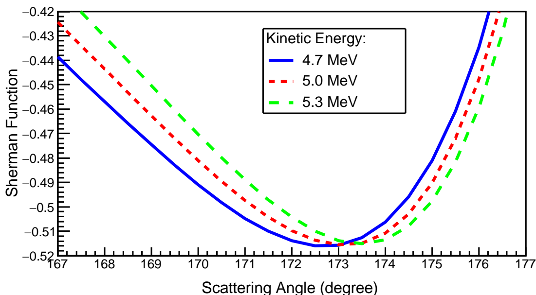
Figure 6. Sherman function for three electron beam kinetic energies.
