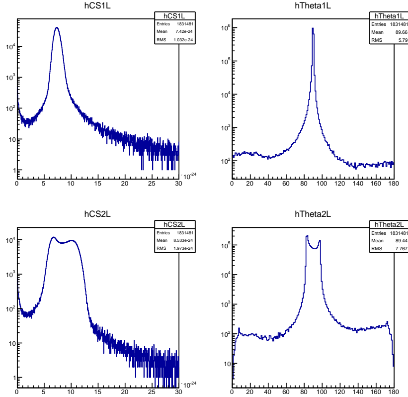
Figure 21. The results for the simulation of double scattering events into one detector arm. The upper plots show the cross-section hCS1L (left) and scattering angle hTheta1L (right) of the first scattering, and the lower plots show the cross-section hCS2L (left) and scattering angle hTheta2L (right) for the second scattering towards the Mott detector. The phi angle was also simulated, but does not alter the simulation results above.
