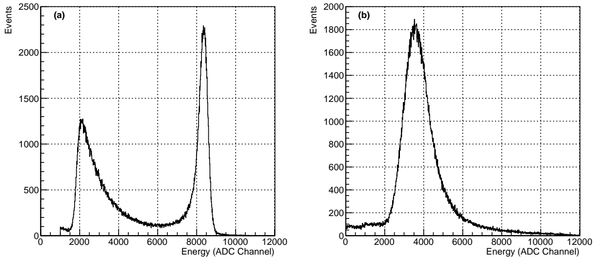
Figure 10. Typical histograms of the (a) E and (b) \Delta E detectors. The E threshold was set to -25 mV for this data and no timing cut was applied. Data from Run 1 with the 350 nm foil.
