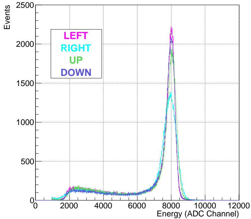
Figure 11. The superimposed normalized energy spectra of the four E detectors, after the timing cut was applied. Data from Run 1 with the 350 nm foil.
