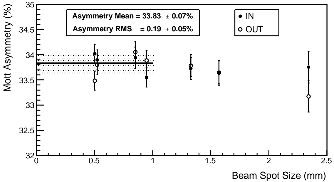
Figure 16. Mott asymmetry vs. beam size
