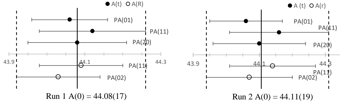
Figure 19. The values of A(0) extrapolated from thickness (solid dots) or rate (open circles) using the Pade approximants are shown for (a) Run 1 and (b) Run 2. The solid vertical line is the average (unweighted) of the A(0) fit parameters, and the vertical dotted lines show the extrema of the uncertainties.
