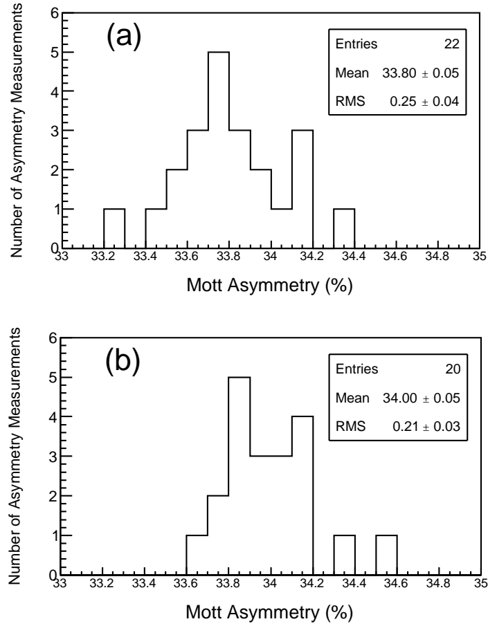
Figure 14. Distribution of asymmetry values of the stability runs. (a) Stability measurements during Run 1 (both low and high discriminator thresholds), (b) Stability measurements during Run 2. The RMS width of the distribution is very close to the statistical uncertainty of the single Mott measurement.
