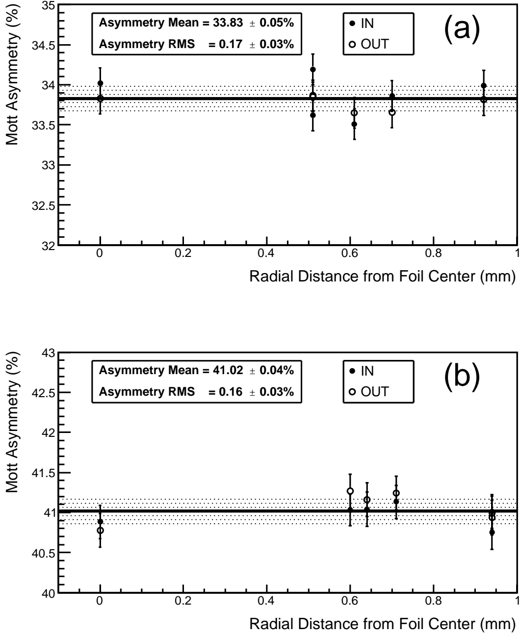
Figure 15. Mott asymmetry vs. radial displacement from the center of the target foil using the (a) 1 \mu\text{m} and (b) 0.225 \mu\text{m} foils
