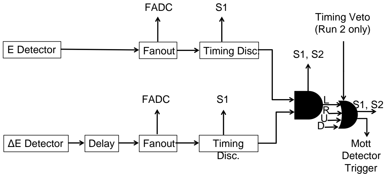
Figure 8. Electronic signal processing of the \Delta E and E signals (the “Left” of four detector arms).
