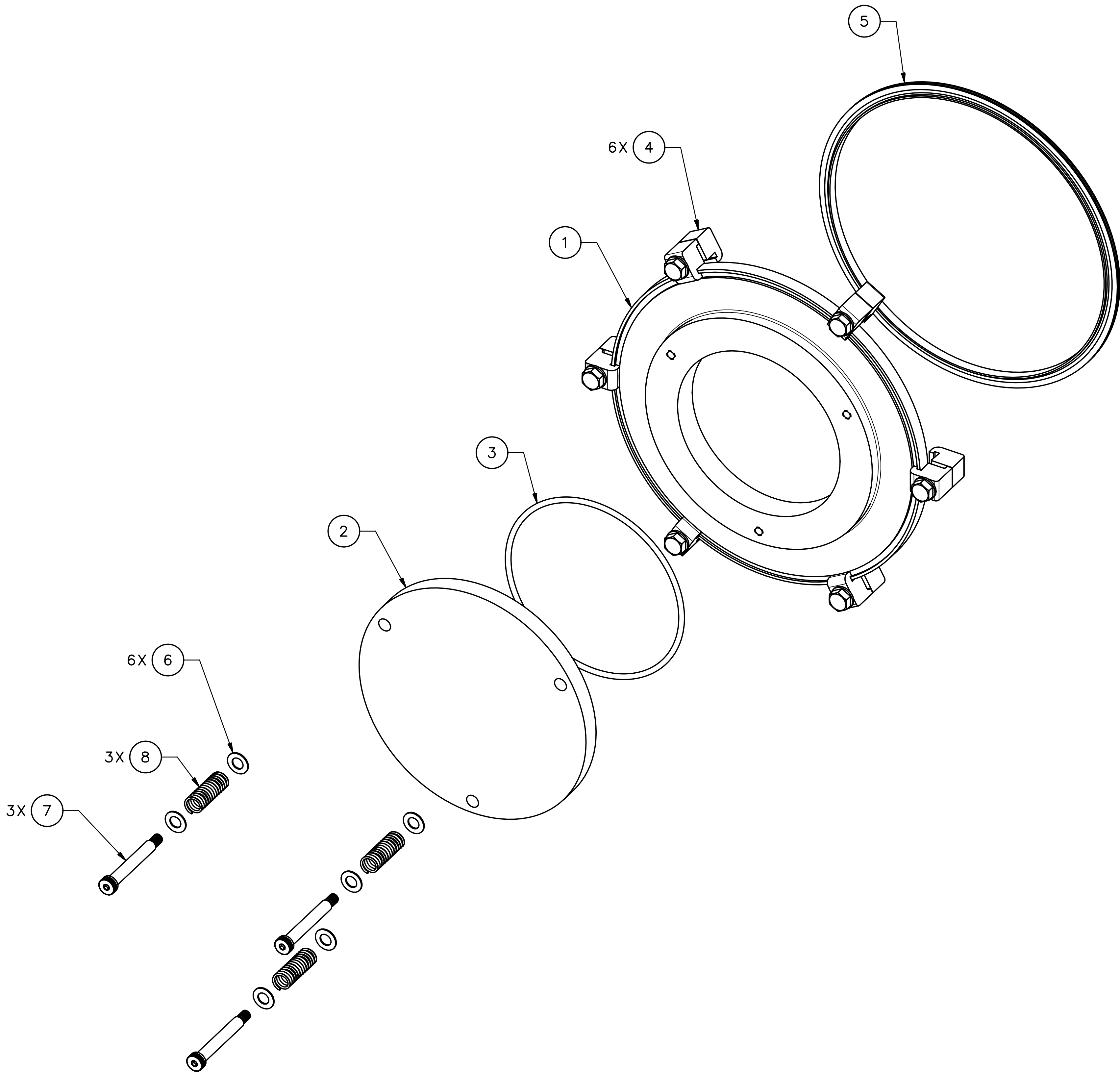
EXPLODED VIEW
