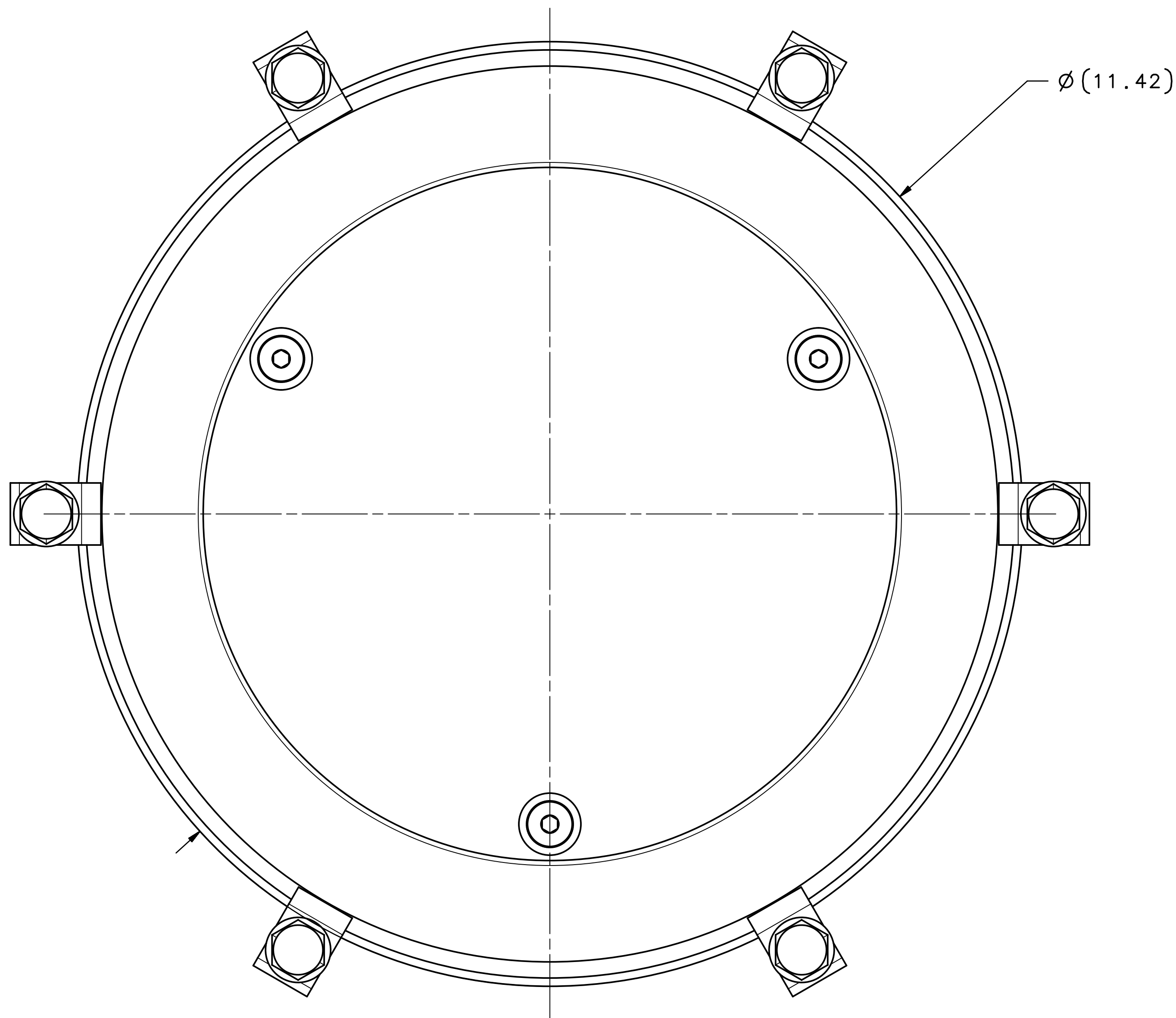
FRONT VIEW
