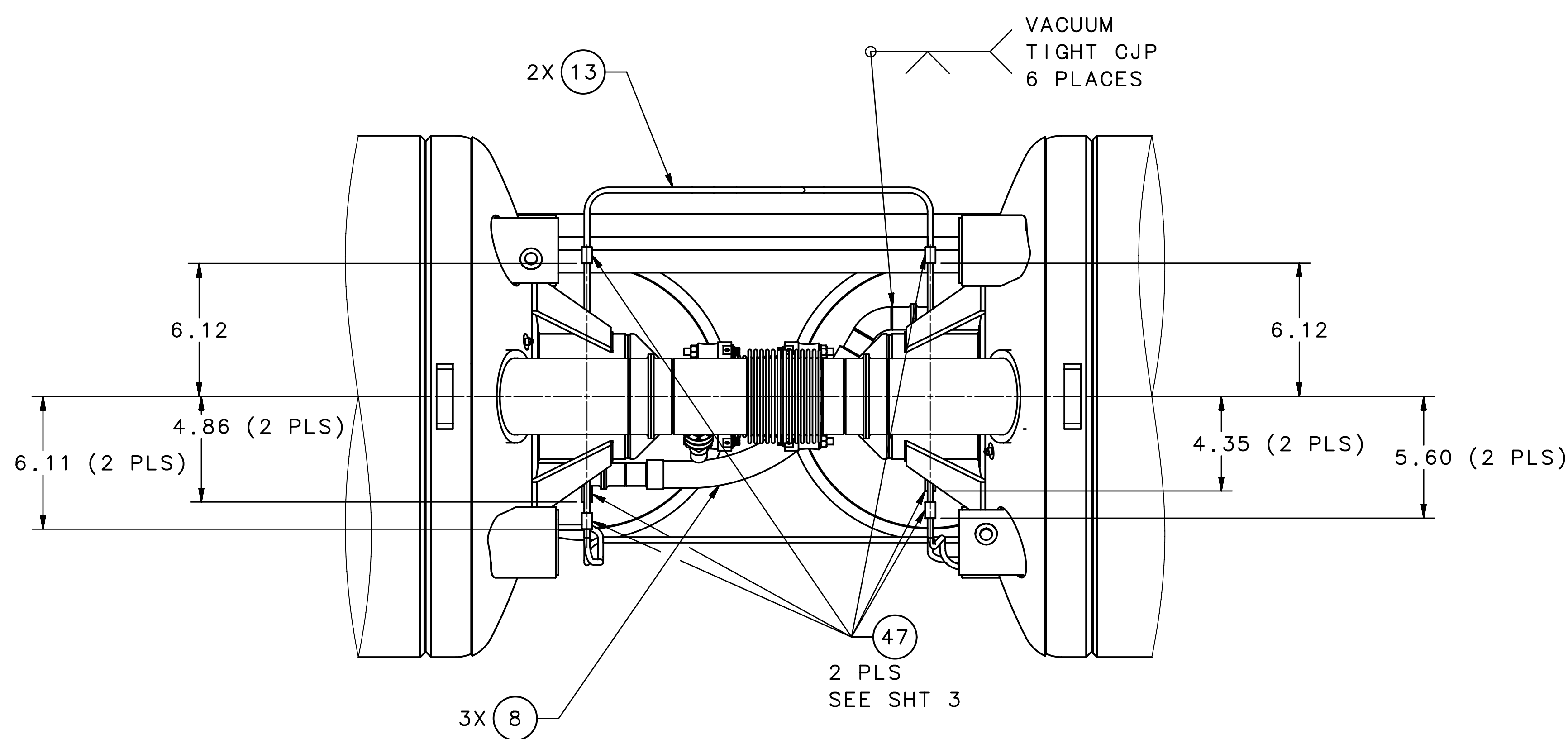
VIEW B-B SCALE 1:4
