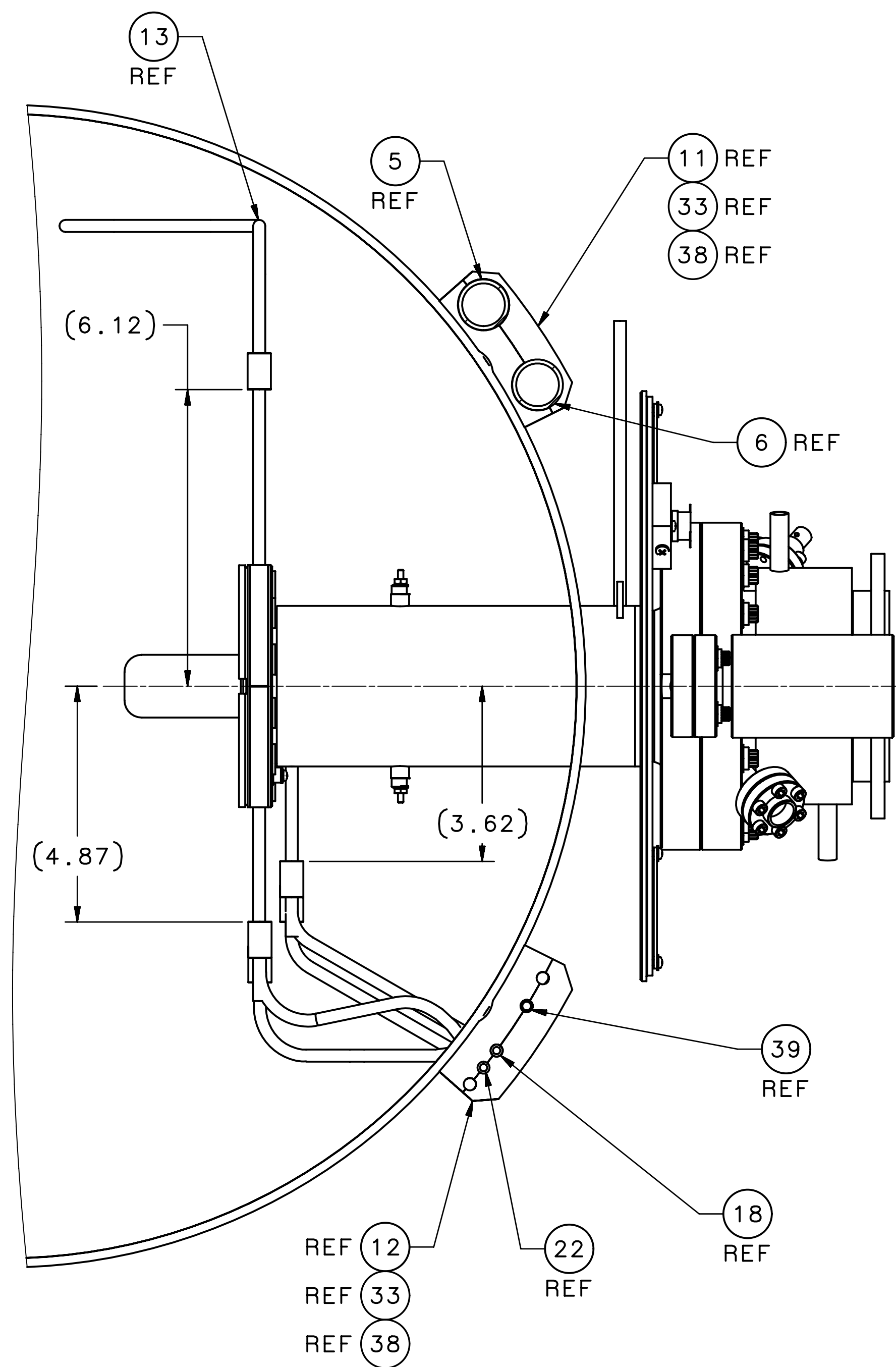
PARTIAL TOP VIEW COUPLER AND HEAT EXCHANGE PIPING
