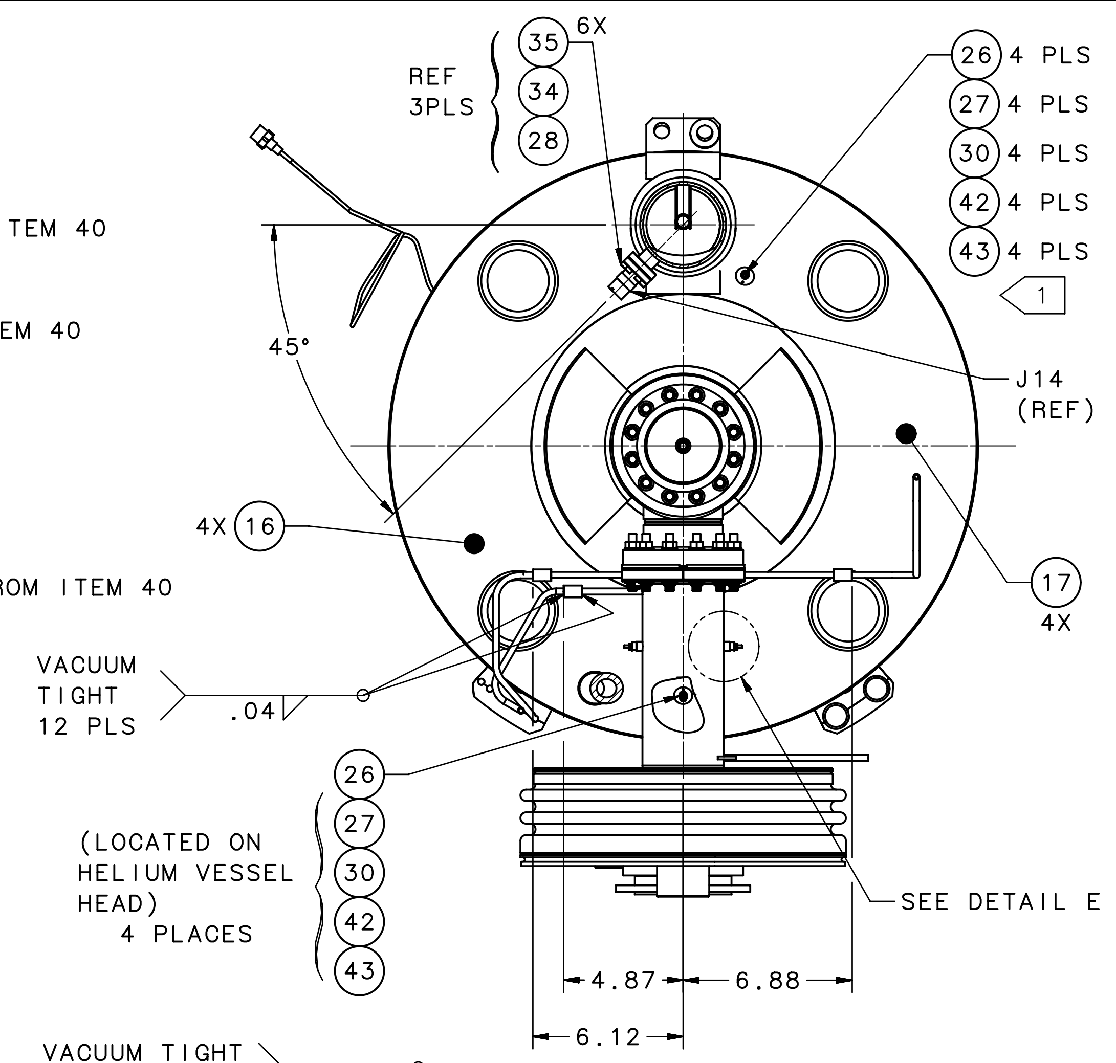
SECTION C-C SCALE 1:4
