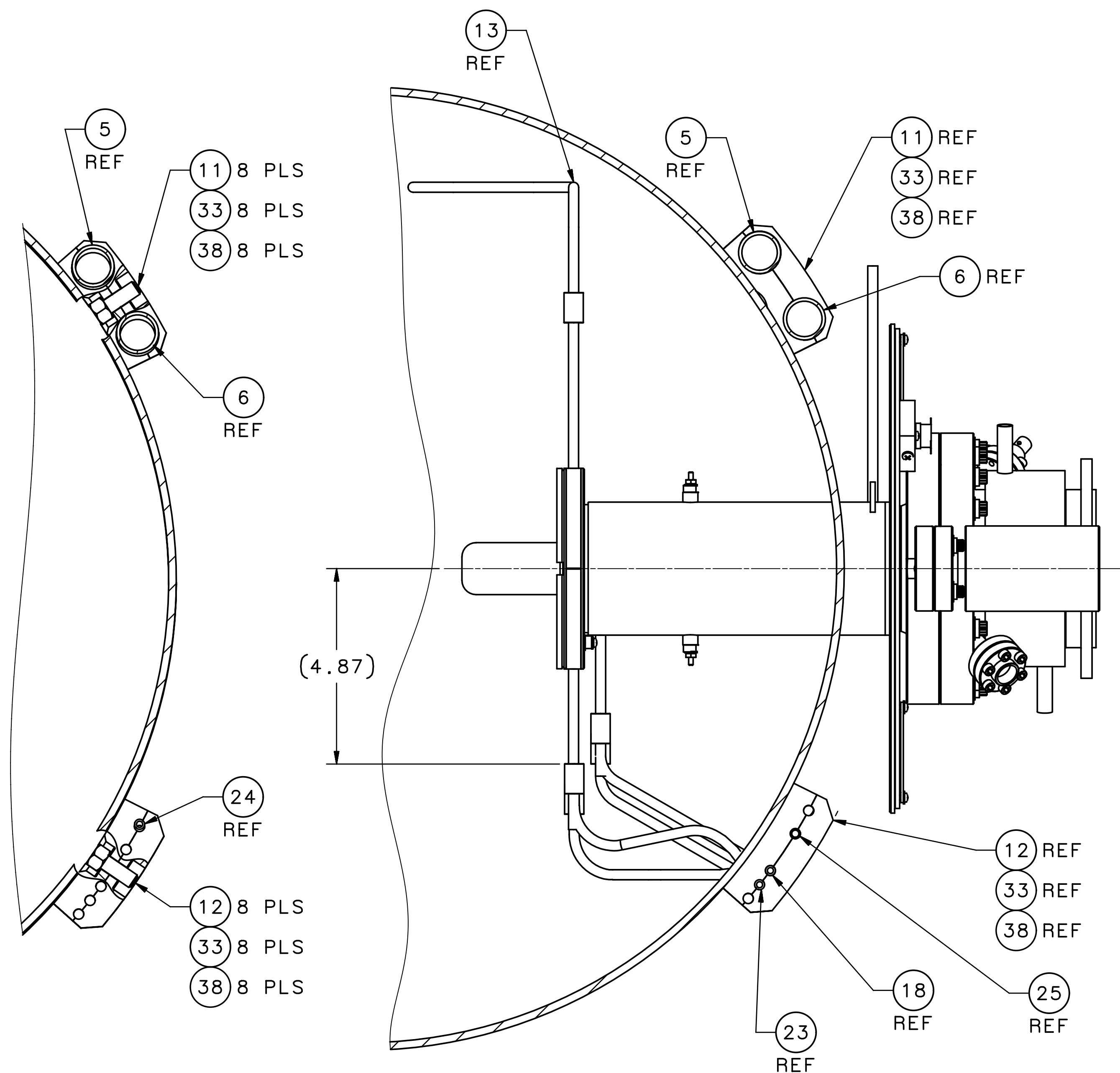
SECTION M-M SCALE 1:2
