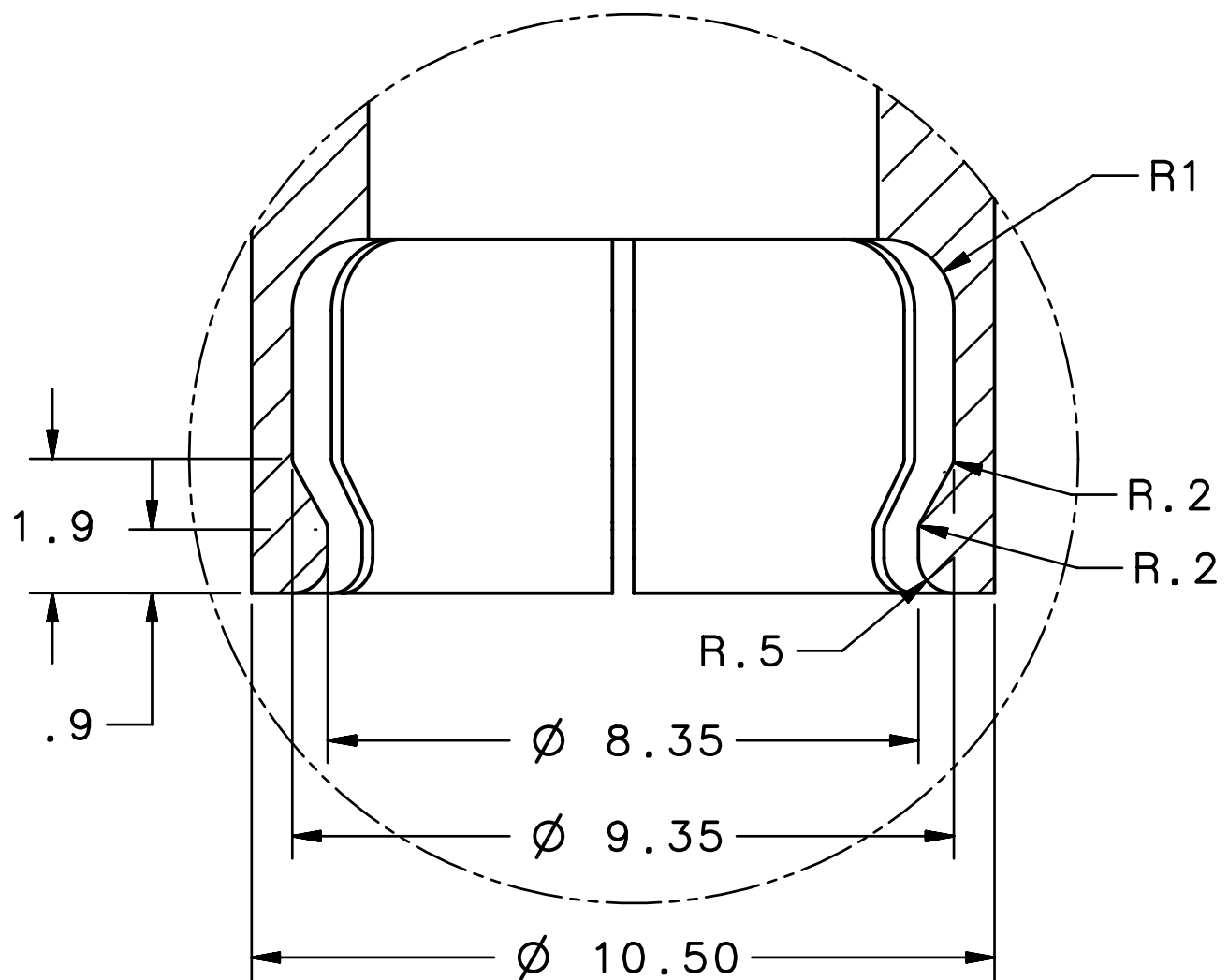
DETAIL B SCALE 10:1
