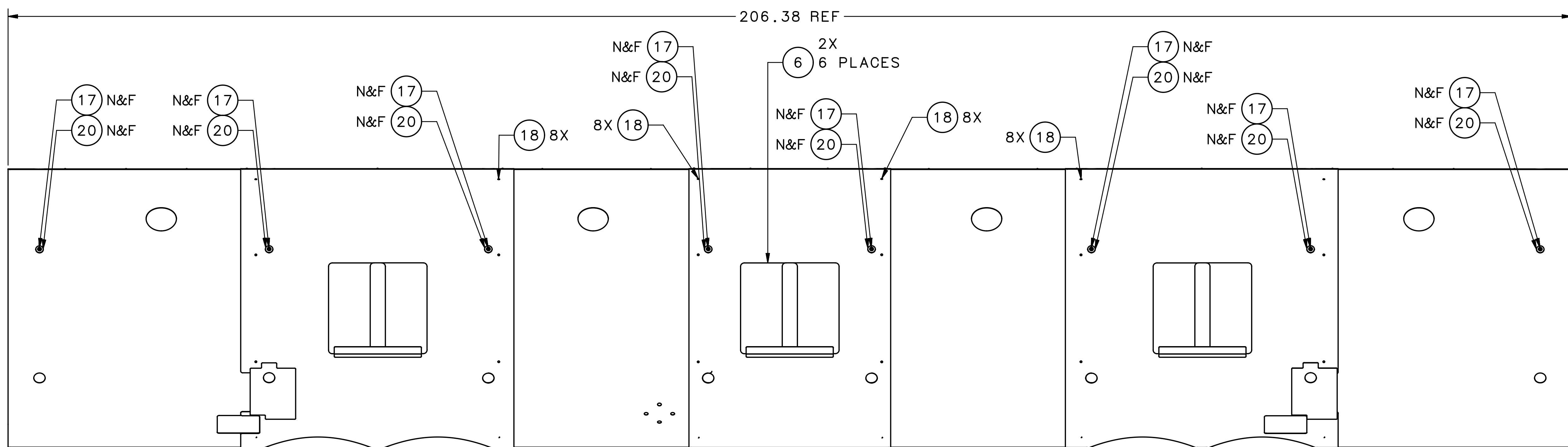
ELEVATION VIEW
