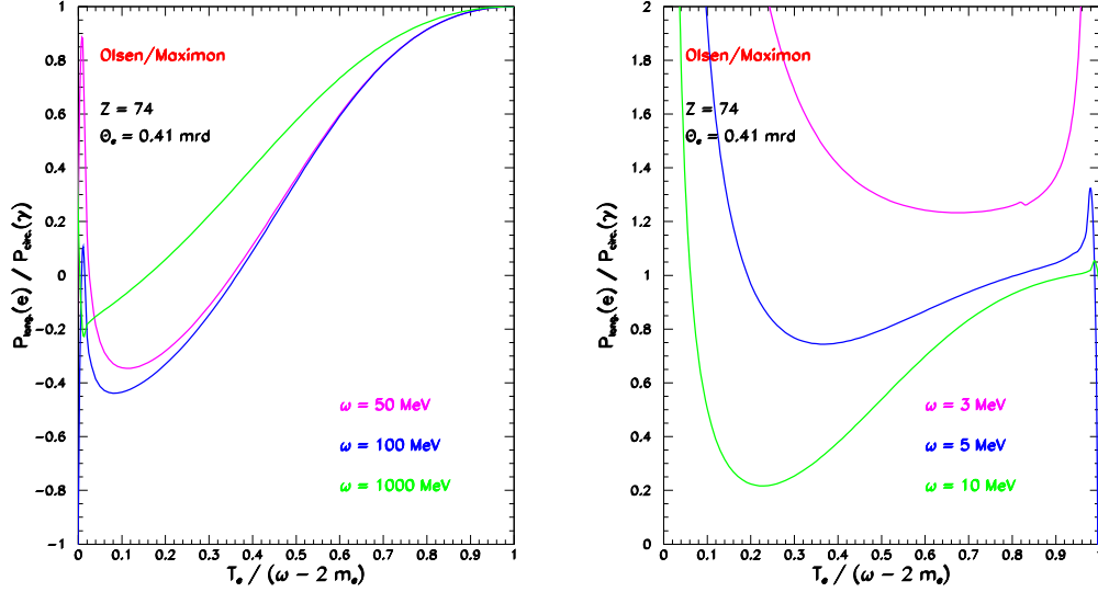
Figure 13. Circular to longitudinal polarization transfer for the pair creation process according to OM prescription at high (left) and low (right) initial photon energy.
