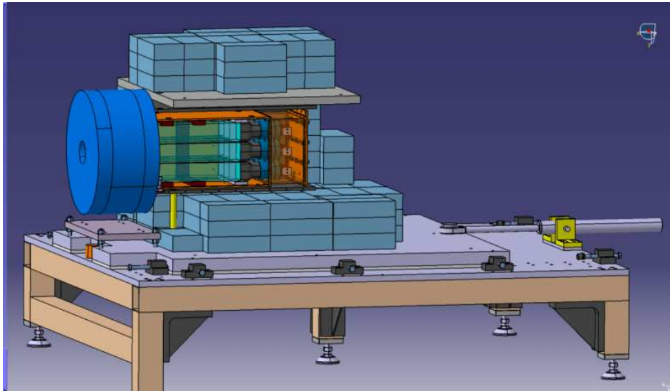
Figure 9. PEPPo positron polarimeter setup
