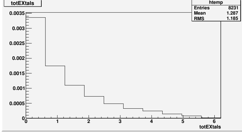
Figure 11. Number of transmitted photons for 10 energy bins and 1 million incident positrons
