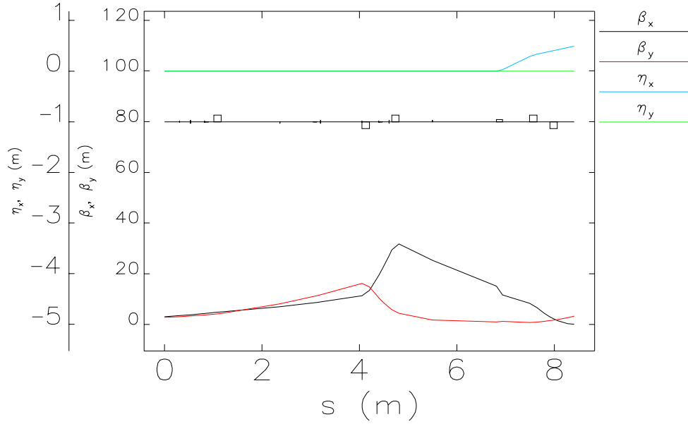
Figure 5. Electron beam optics along the PEPPo Region 0 and 1 to obtain a beam diameter of 3 mm at the first target. Here the beamline starts from 0.3 m upstream from the first viewer (ITV0L01) in the Region 0, and three quadrupoles in Region 0 are located at s \simeq 1.2 m, 4.2 m, and 4.8 m. The MBV0L021 dipole is located at s \simeq 6.9 m, and two new quadrupoles are located at s \simeq 7.6 m and 8.1 m. The first target is located at the end of the beamline, s \simeq 8.4 m.
