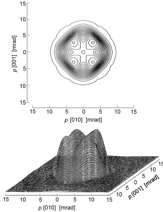
Figure 18. Two-dimensional angular correlation of annihilation radiation in gallium arsenide exhibiting no positron trapping in defects [Tan95].
