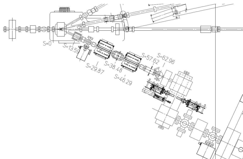
Figure 3. Layout of the Region 1 of the PEPPo beamline. Here the beamline is rotated by -90 degree from the layout in Fig. 2.
