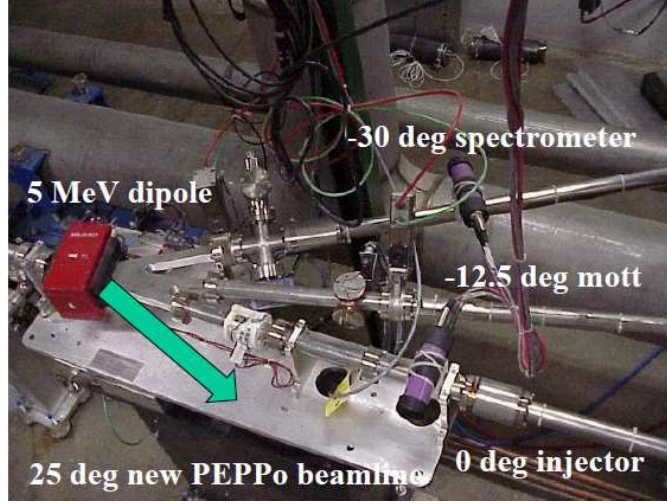
Figure 4. Three existing beamlines and a new PEPPo beamline of a dipole (MBV0L021).
