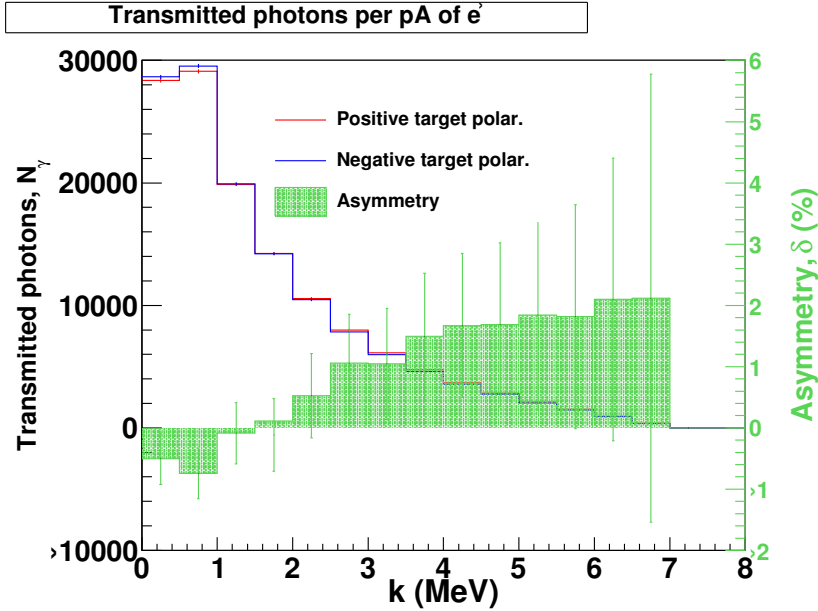
Figure 10. Number of transmitted photons for two opposite target polarization and expected experimental asymmetry as obtained from GEANT4 simulations. The statistical error bars correspond to a data taking time of 1 s at a 1 pA current.
