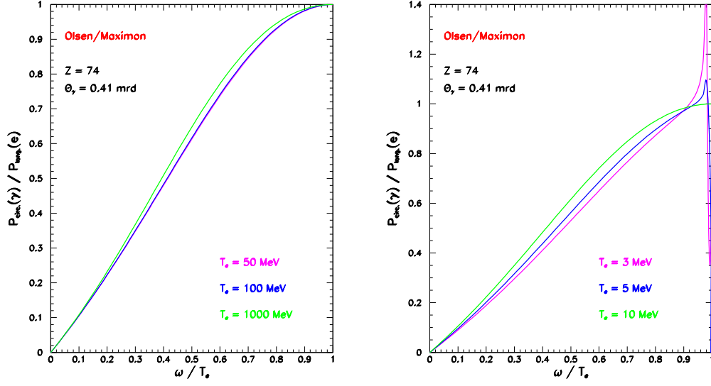
Figure 12. Longitudinal to circular polarization transfer for the bremsstrahlung process according to OM prescription at high (left) and low (right) initial electron kinetic energy.
