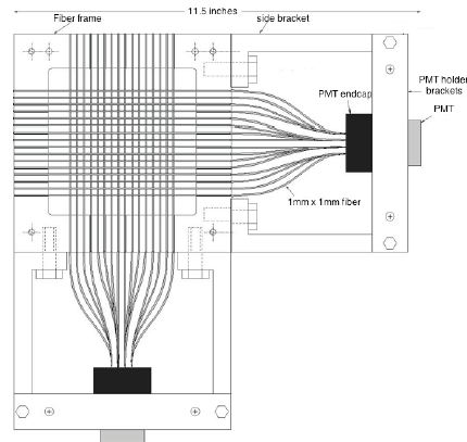
Figure 7. The 32 channel scintillating fiber monitor used in the two-photon exchange experiment in Hall B [?]
