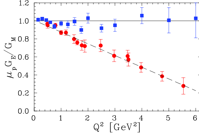
Figure 26. most recent experimental data on the electromagnetic form factor ratio as measured from polarization transfer [Jon00,Gay02,Puc10] and Rosenbluth separation [And94,Chr04,Qat05] experiments.
