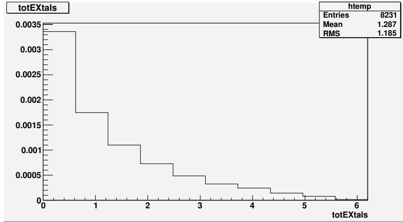
Figure 20. Number of transmitted photons for 10 energy bins and 1 million incident positrons
