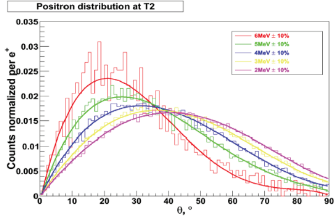
Figure 16. Positrons phase space.
