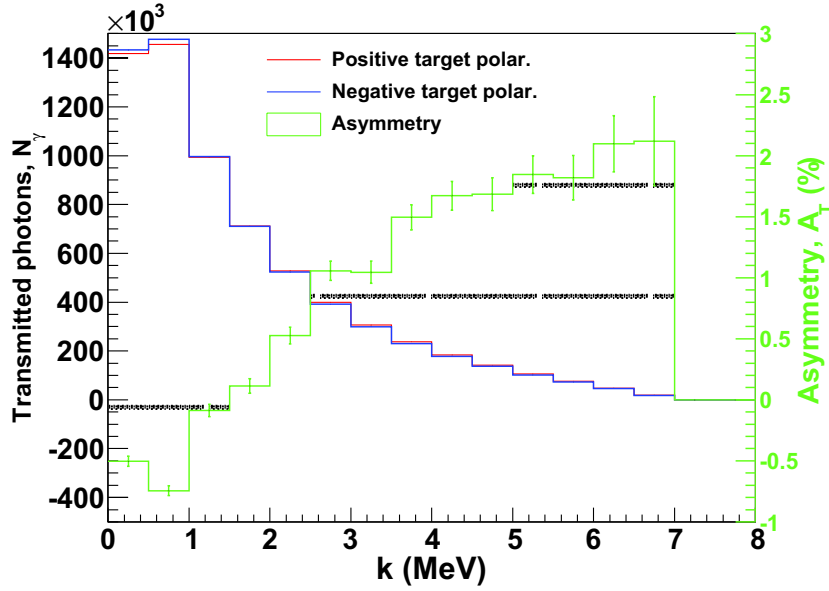
Figure 19. Number of transmitted photons for two opposite target polarizations and expected experimental asymmetry as obtained from G4PEPPo simulations for 000 incident positrons ( T_e = 6 MeV, P_t = 100 %, P_e = \pm 100 %).
