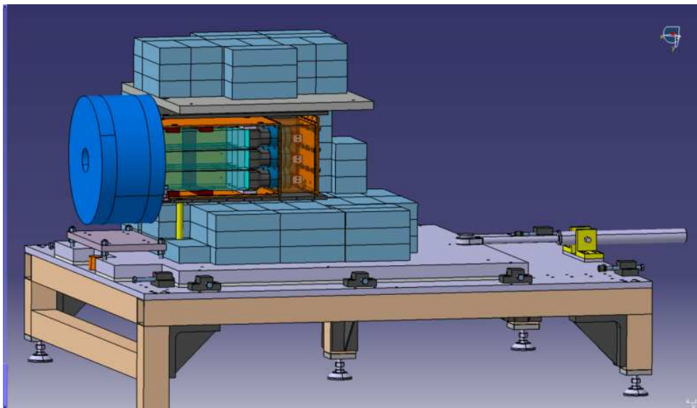
Figure 7. PEPP0 positron polarimeter setup
