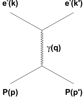
Figure 22. lowest order (QED) diagram of the elastic eP reaction; the initial and final electron momentum four-vectors are k and k' , respectively, and p and p' for the proton; the four-momentum transfer to the photon is q .
