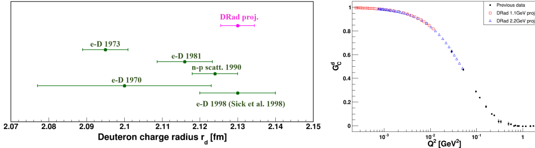
Figure 1: (left) The projected radius result along with other electron scattering measurements. (right) Projected charge form factor along with existing data.
