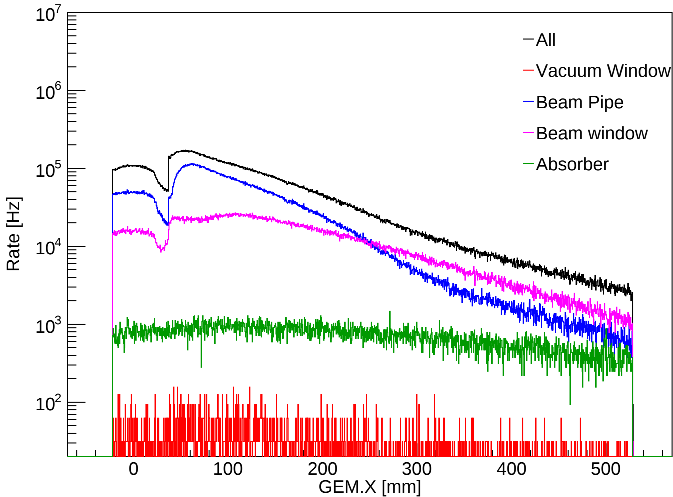
He pipe GEM Background Rate in each strips [DID==2]
