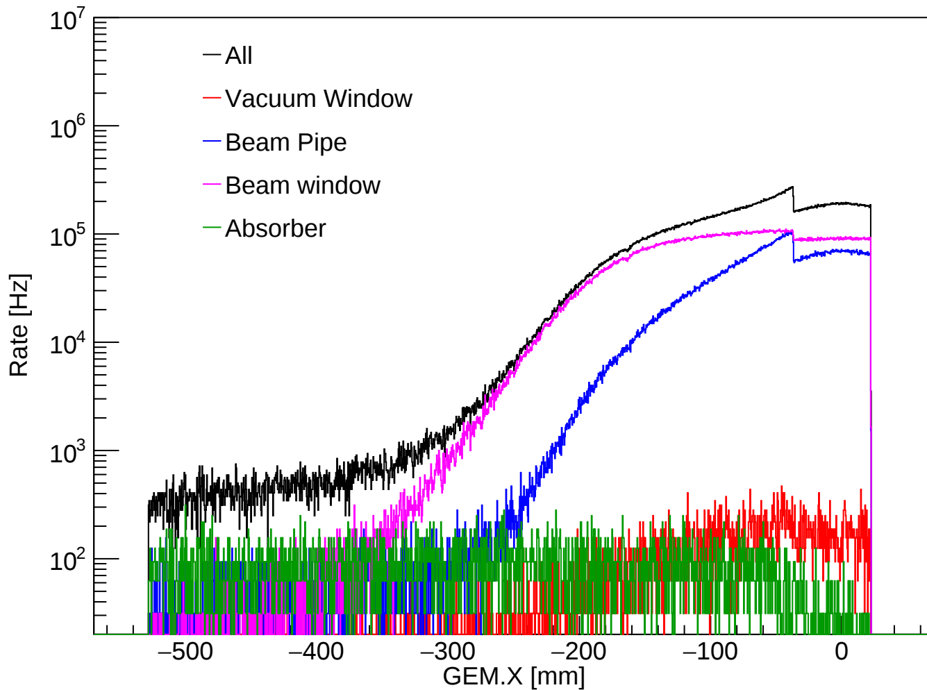
He pipe GEM Background Rate in each strips [DID==1]
