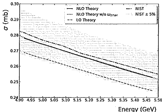
FIG. 3: Comparison of theoretical calculations of total Compton cross section using different approaches. The solid and the dotted curves are calculated by two different numerical methods - described in the text. The dotted-dashed line represents the NIST calculation - XCOM code. The dashed curve is calculated using the Klein-Nishina formula.
