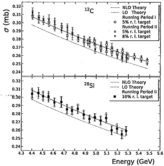
FIG. 6: The Compton cross sections measured on atomic electrons of ^{12}\text{C} and ^{28}\text{Si} targets. The dashed curve corresponds to the Klein-Nishina calculation. The solid curve is the result of next-to-leading order calculation. Bold gray error bars are systematic uncertainties and thin black error bars are statistical uncertainties.
