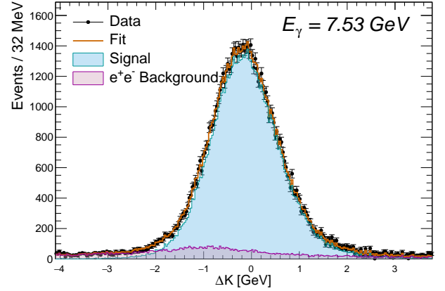
Figure 3: Example of a fit to the \Delta K distribution to extract the Compton yield in one bin of the energy E_\gamma of the (tagged) beam photon (here: 7.53 GeV). See Eq. ?? for the definition of \Delta K . Backgrounds from beam-line components and accidentals in the photon tagger have already been subtracted. The remaining background (shown in magenta) is estimated from simulation of e^+e^- pair production in the target, and the signal line shape (blue) is estimated from the simulation of the Compton scattering signal.
