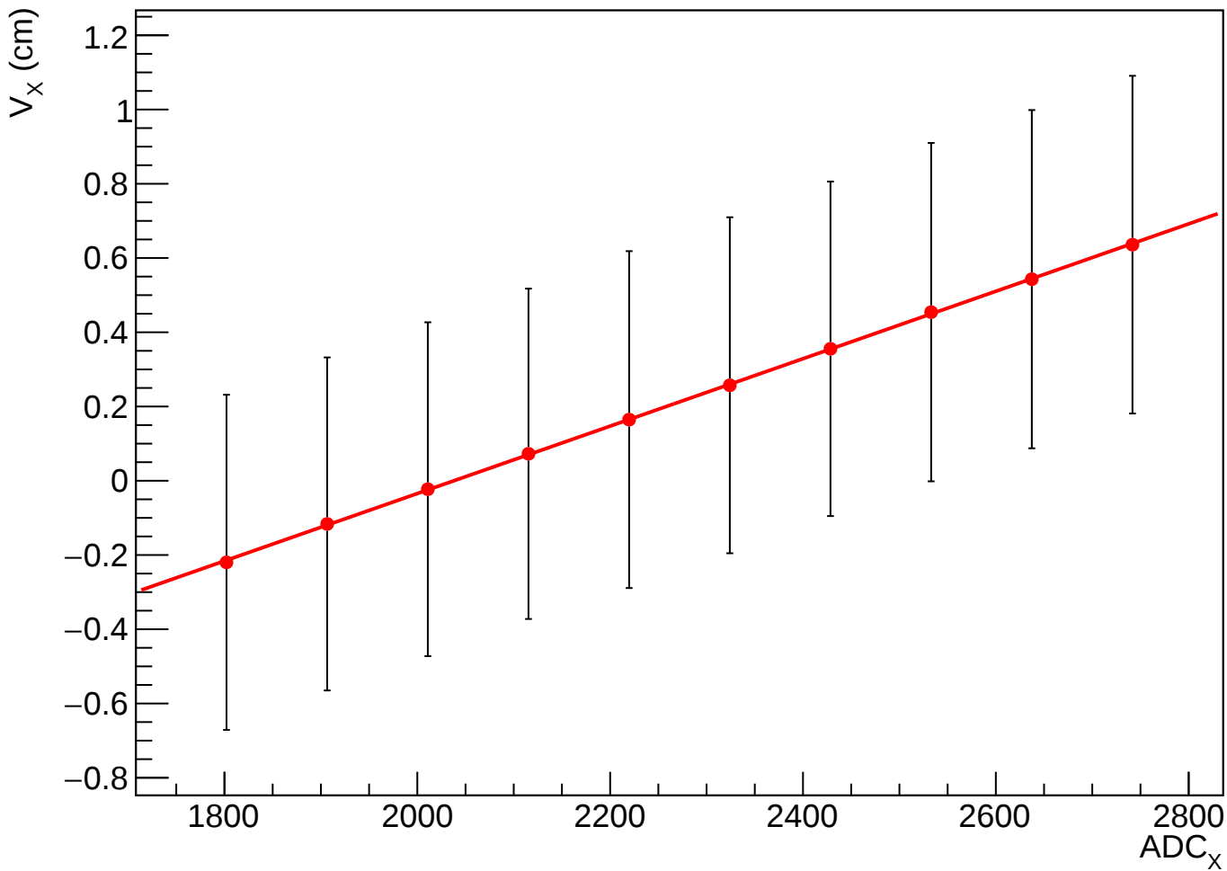
Vertex Position V_x vs. ADC_x
