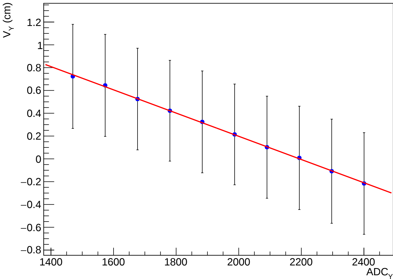
Vertex Position V_Y vs. ADC_Y
