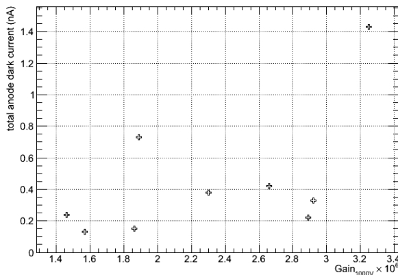
Figure 1: Dark current as a function of MAPMT gain.
