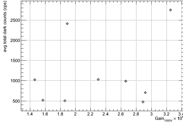
Figure 2: Average dark count rate as a function of MAPMT gain.
