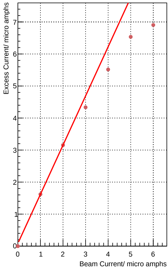
INFN_J2_Middle || 3.7 GeV || BB at 36.0 degrees || LH2 target
