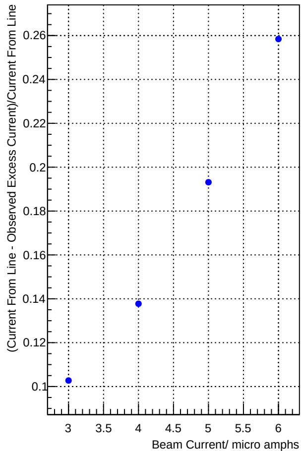
INFN_J0_Bottom || 3.7 GeV || BB at 36.0 degrees || LH2 target
