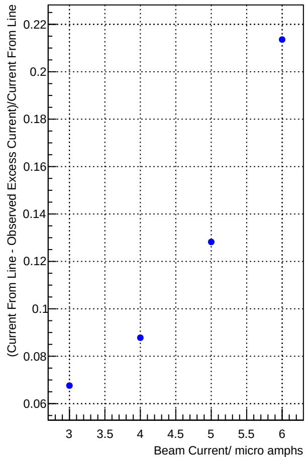
INFN_J2_Bottom || 3.7 GeV || BB at 36.0 degrees || LH2 target
