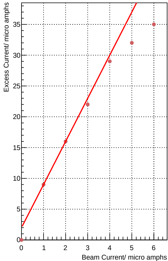
UVA_UV_Layer1 || 3.7 GeV || BB at 36.0 degrees || LH2 target
