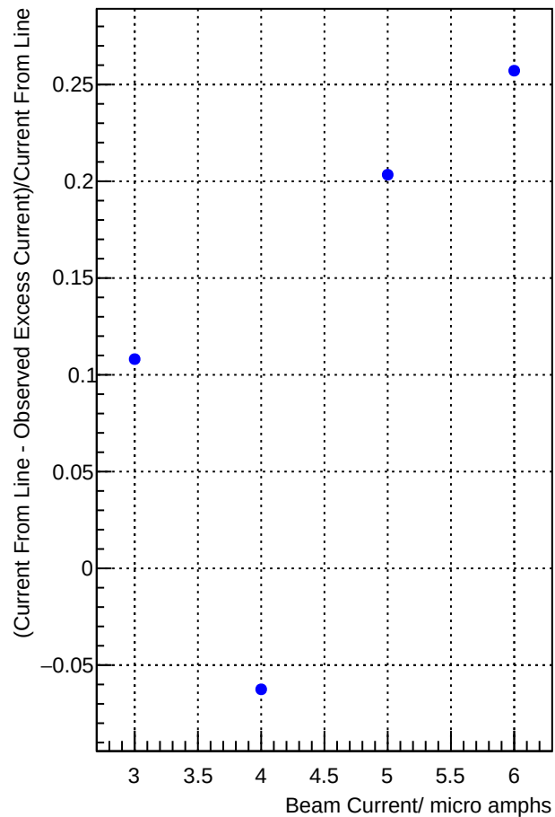
UVA_UV_Layer0 || 3.7 GeV || BB at 36.0 degrees || LH2 target
