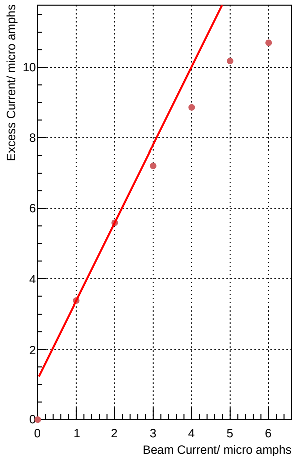
INFN_J0_Middle || 3.7 GeV || BB at 36.0 degrees || LH2 target
