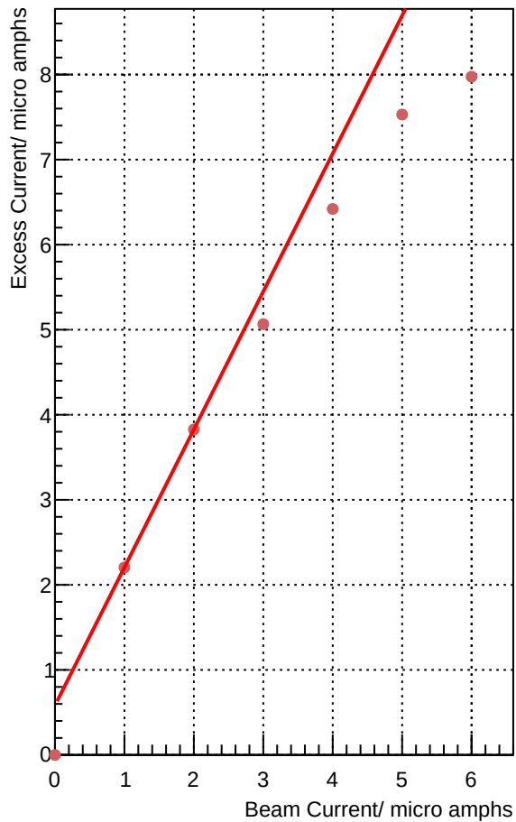
INFN_J0_Top || 3.7 GeV || BB at 36.0 degrees || LH2 target
