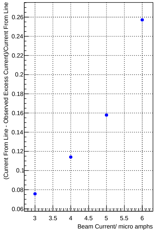
INFN_J2_Middle || 3.7 GeV || BB at 36.0 degrees || LH2 target
