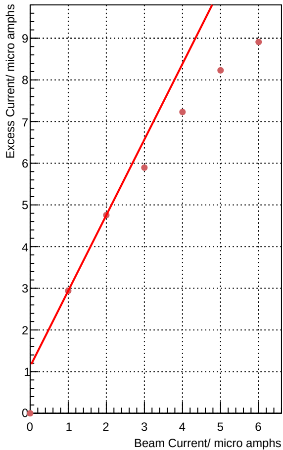
INFN_J0_Bottom || 3.7 GeV || BB at 36.0 degrees || LH2 target
