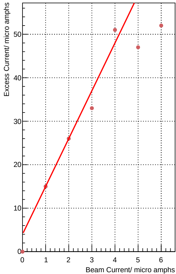
UVA_UV_Layer0 || 3.7 GeV || BB at 36.0 degrees || LH2 target
