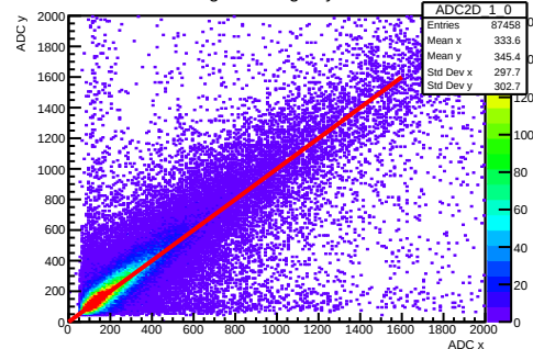
Cluster Charge Sharing Layer 1 Module 0
