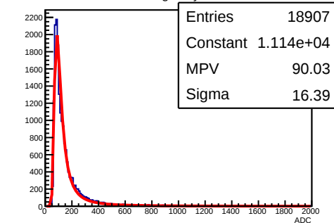
X Cluster Charge Layer 1 Module 2
