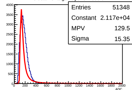
X Cluster Charge Layer 3 Module 2
