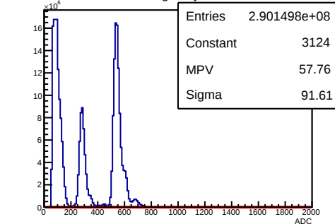
X Cluster Charge Layer 1 Module 0
