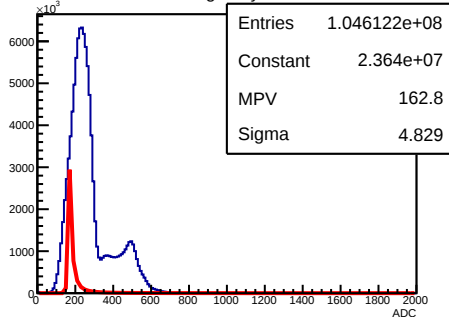
X Cluster Charge Layer 1 Module 1
