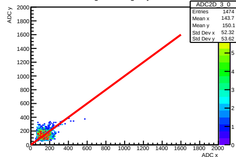
Cluster Charge Sharing Layer 3 Module 0
