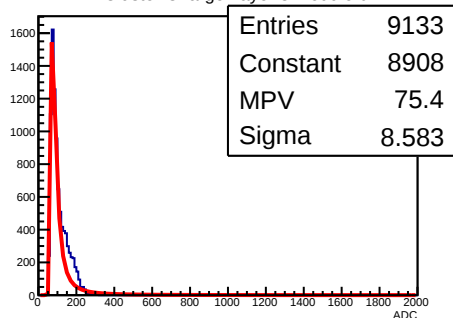
X Cluster Charge Layer 3 Module 0
