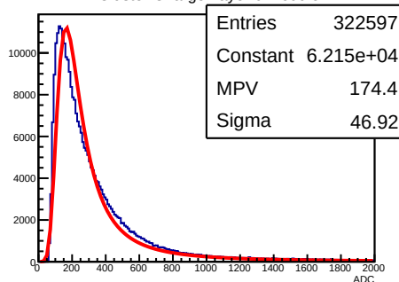
X Cluster Charge Layer 0 Module 1
