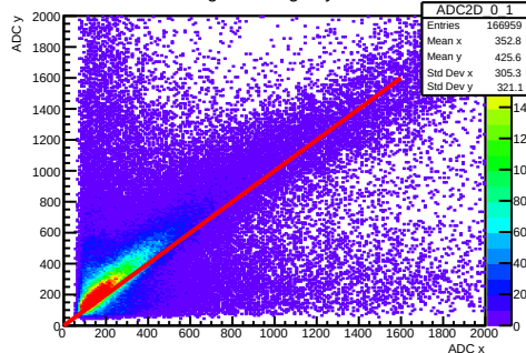
Cluster Charge Sharing Layer 0 Module 1
