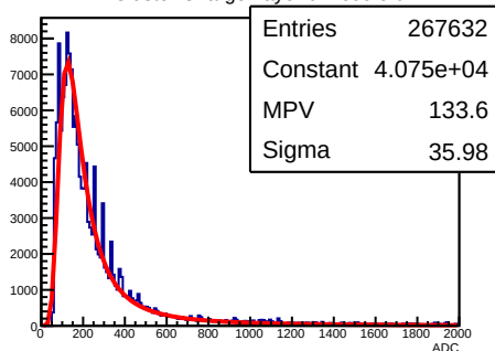
X Cluster Charge Layer 0 Module 0
