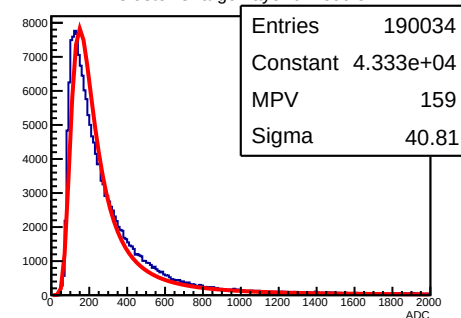
X Cluster Charge Layer 0 Module 2
