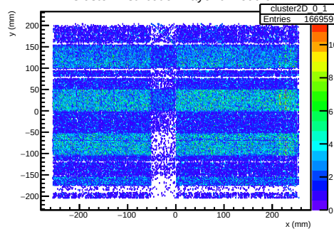
Cluster Distribution Layer 0 Module 1
