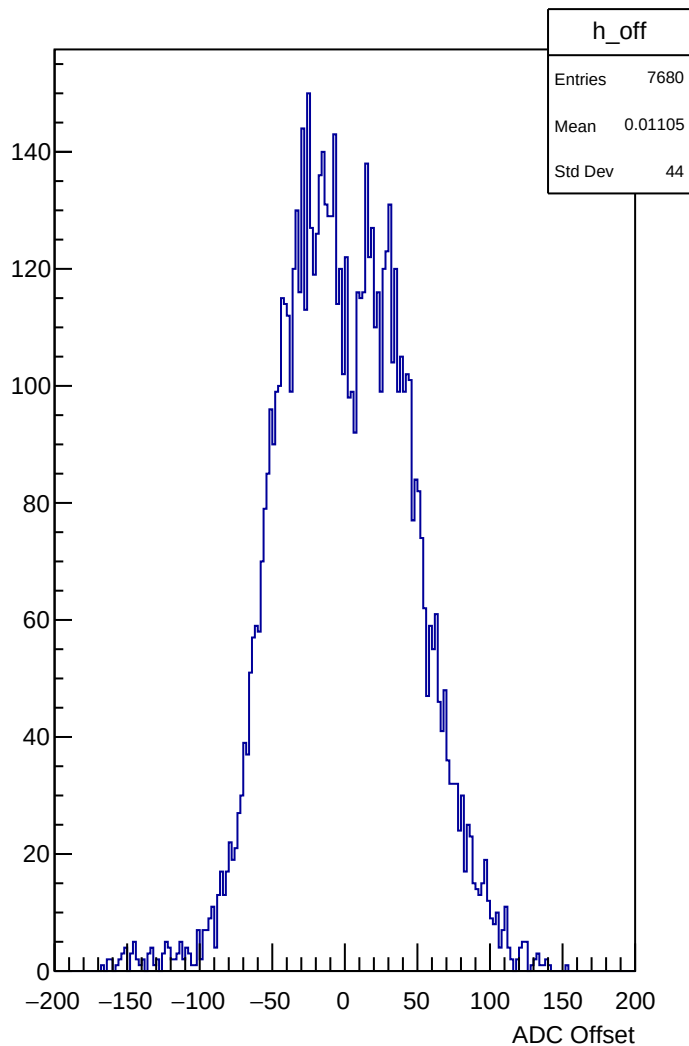
Offset of All Channels
