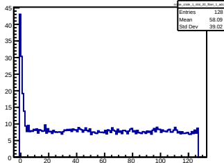
noise_crate_1_slot_20_fiber_1_adc_1
