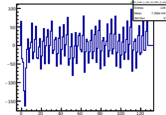
offset_crate_1_slot_20_fiber_0_adc_3
