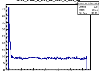
noise_crate_1_slot_20_fiber_0_adc_12
