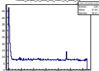
noise_crate_1_slot_20_fiber_0_adc_10
