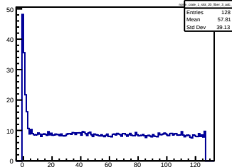
noise_crate_1_slot_20_fiber_3_adc_10
