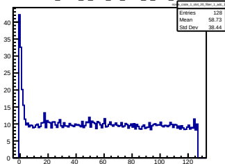
noise_crate_1_slot_20_fiber_1_adc_12
