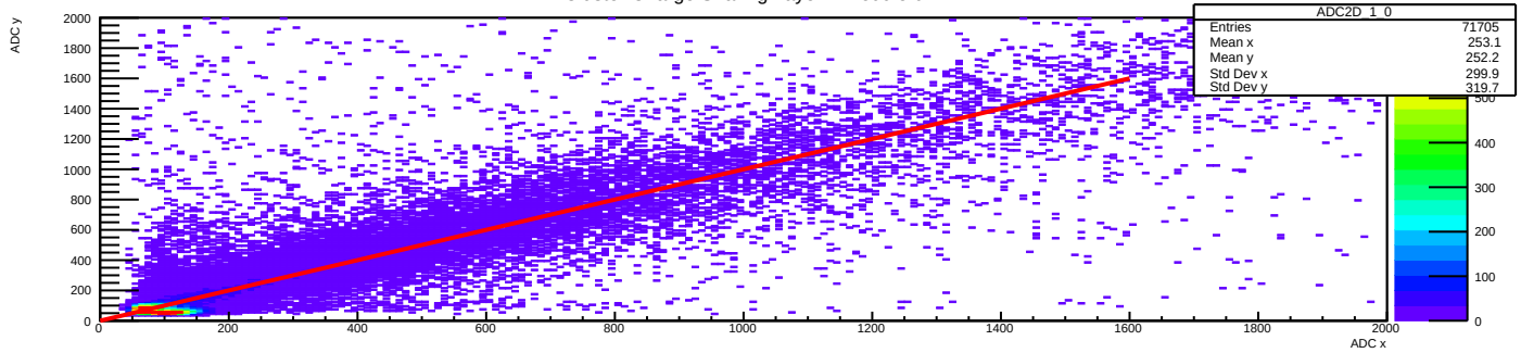
Cluster Charge Sharing Layer 1 Module 0
