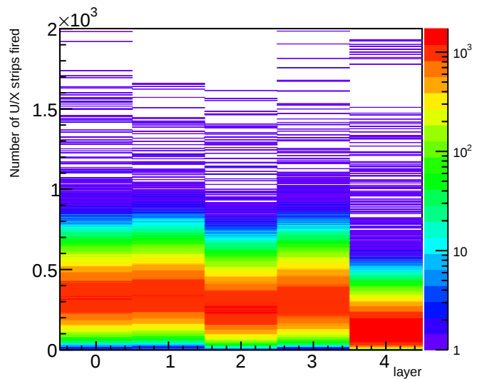
Summary Plots(Run #13240) 0: Strip and cluster multiplicities
