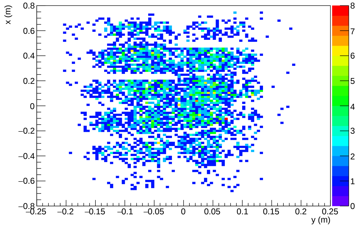
Hits with Peak in Sample 5 Layer 1
