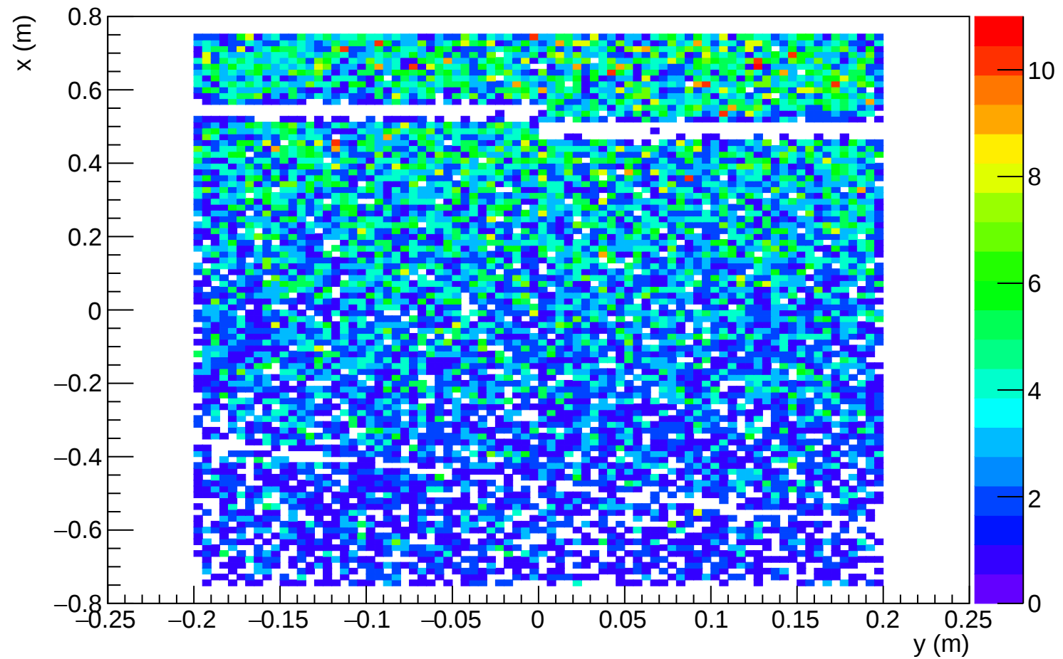
Hits with Peak in Sample 2 Layer 0
