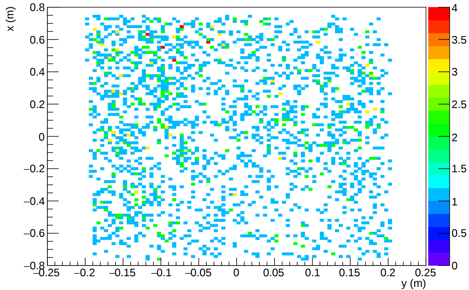
Hits with Peak in Sample 0 Layer 2
