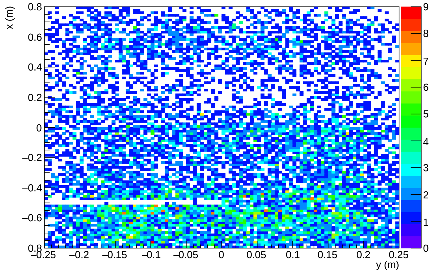
Hits with Peak in Sample 1 Layer 4
