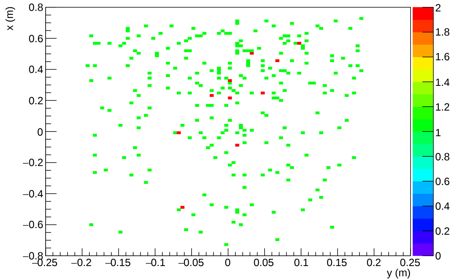
Hits with Peak in Sample 4 Layer 2
