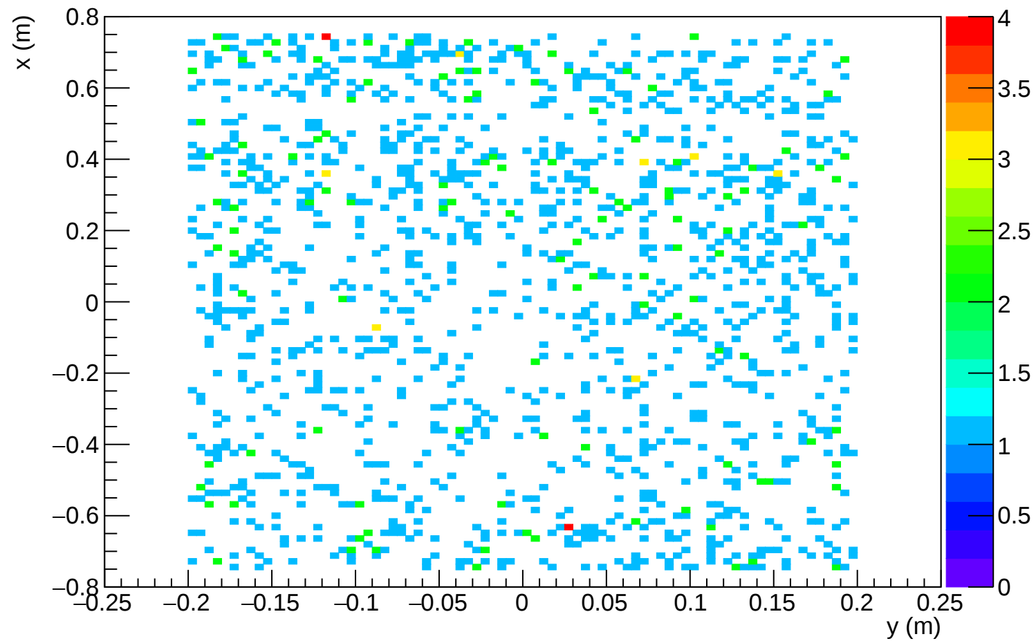
Hits with Peak in Sample 0 Layer 0
