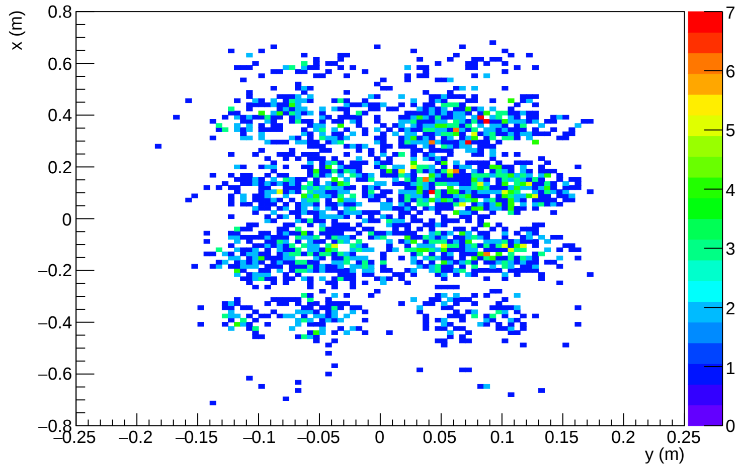
Hits with Peak in Sample 5 Layer 3
