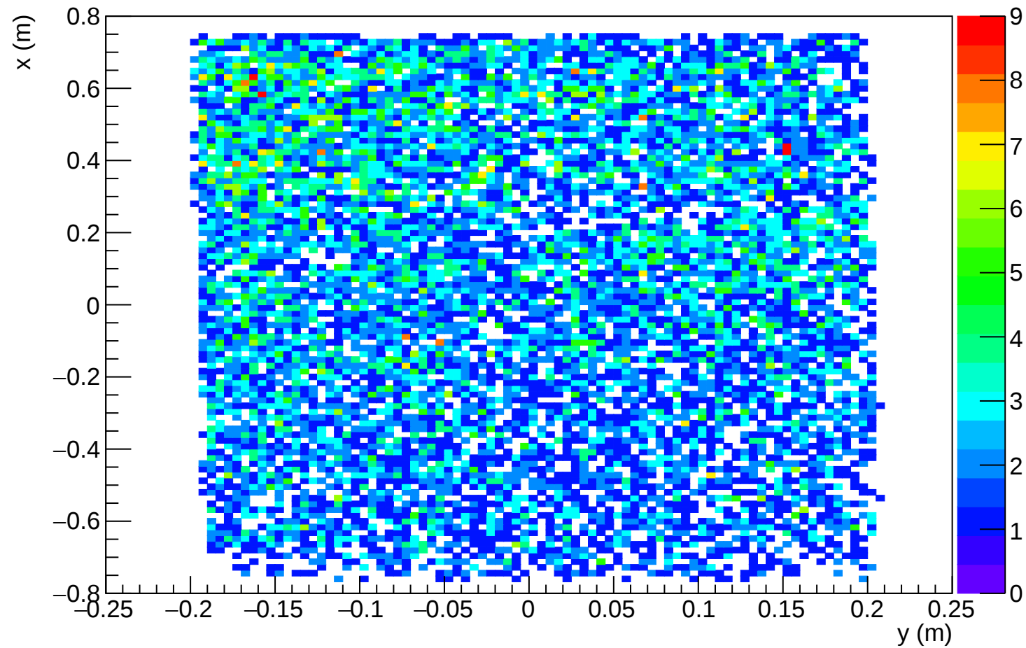
Hits with Peak in Sample 1 Layer 2
