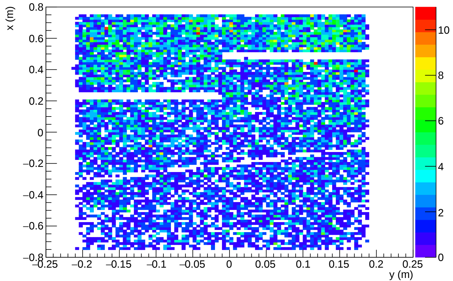
Hits with Peak in Sample 3 Layer 1
