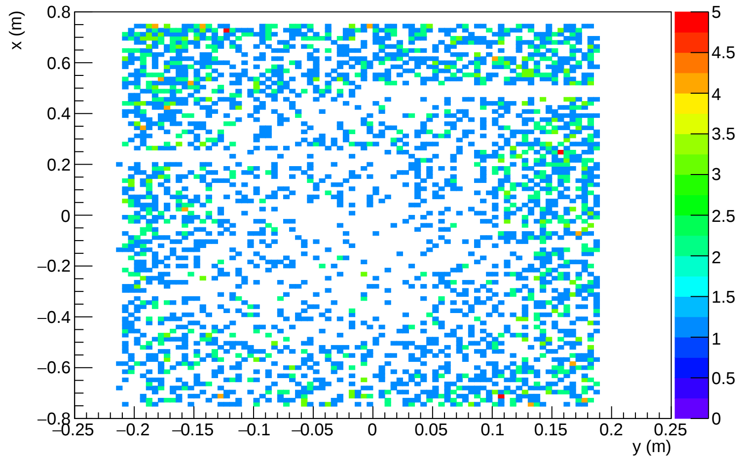
Hits with Peak in Sample 1 Layer 1
