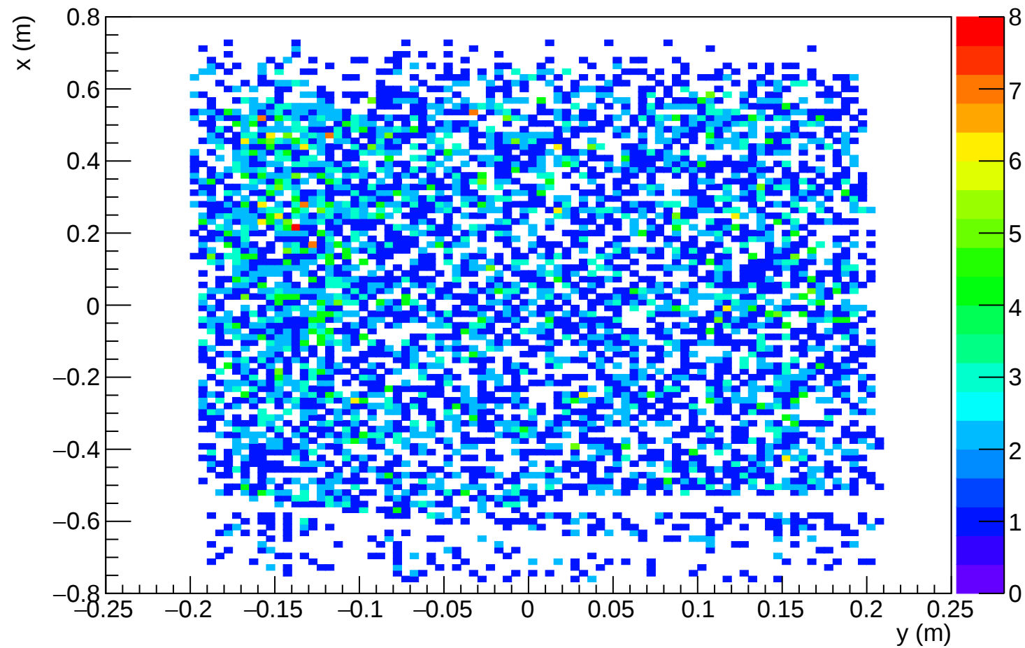
Hits with Peak in Sample 1 Layer 3
