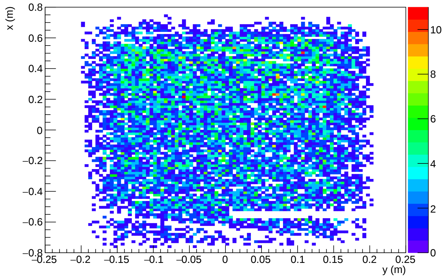
Hits with Peak in Sample 3 Layer 3
