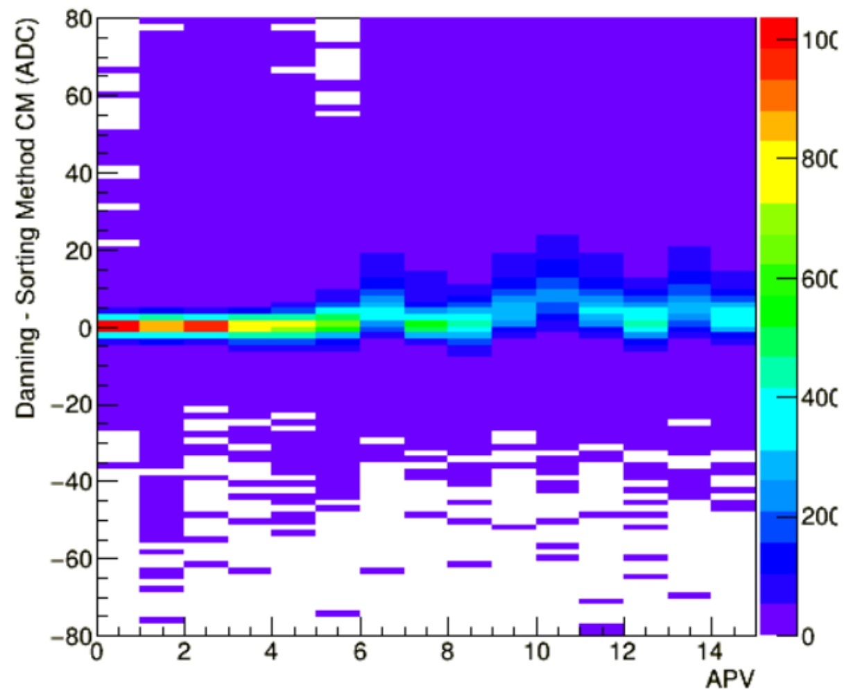
Common Mode Method Comparison
