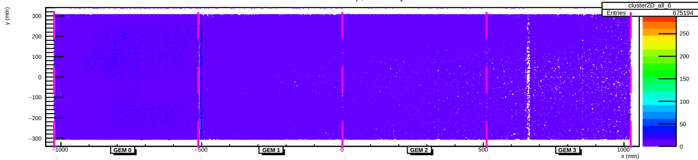
Cluster Distribution Map, Inline Layer 6
