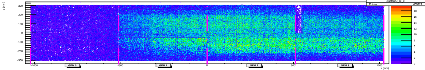
Cluster Distribution Map, PolR Layer 0
